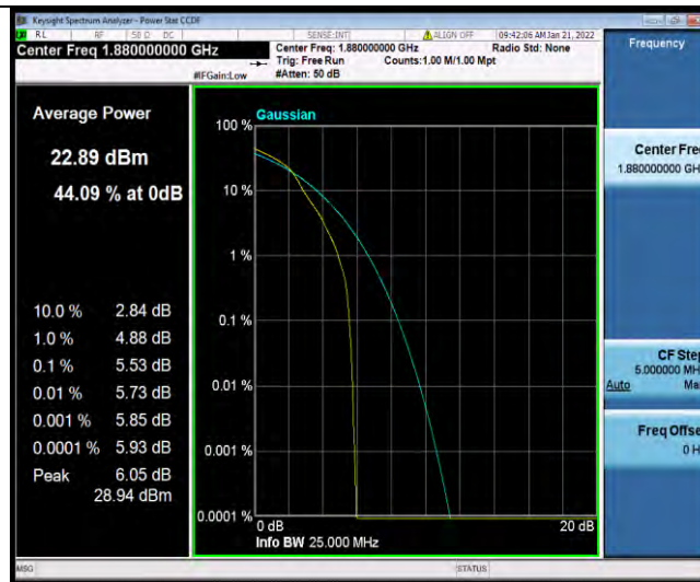
Band2-10MHz-64QAM-18900-50RB#0
