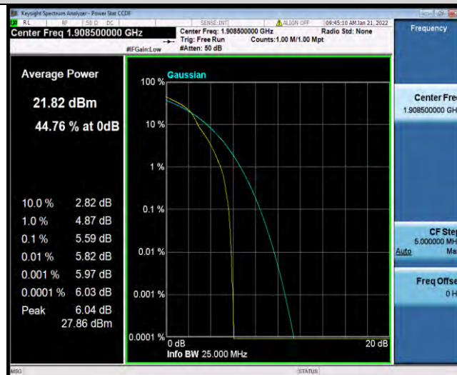
Band2-3MHz-64QAM-19185-15RB#0
