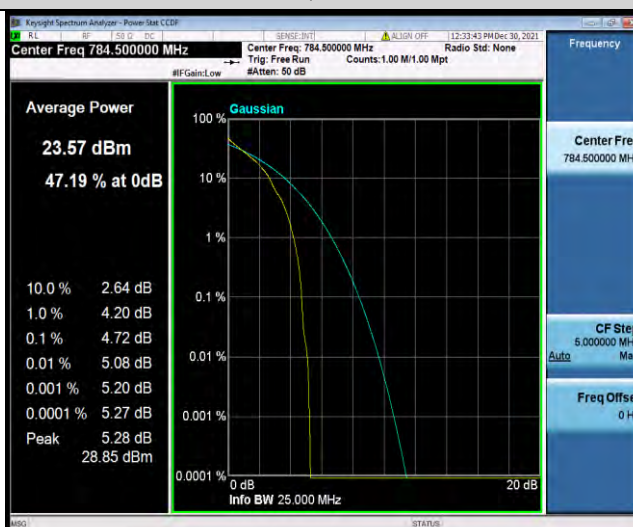
Band13-5MHz-QPSK-23255-25RB#0
