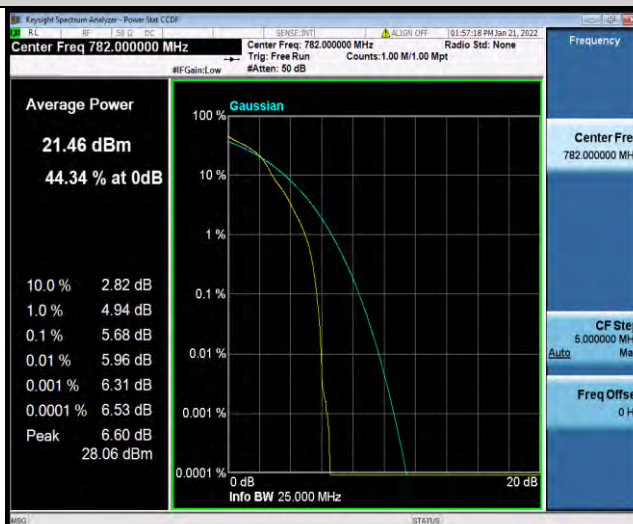
Band13-10MHz-64QAM-23230-50RB#0
