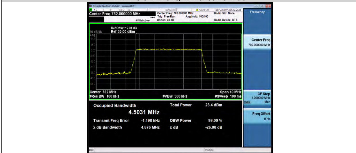
Band13-5MHz-64QAM-23255-25RB#0
