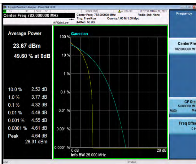
Band13-5MHz-QPSK-23230-25RB#0
