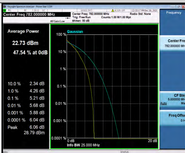
Band13-5MHz-QPSK-23255-1RB#0
