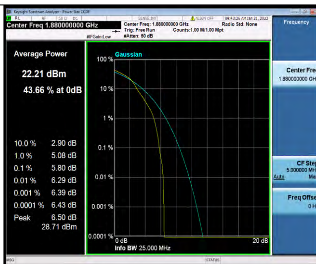
Band2-5MHz-64QAM-18900-25RB#0
