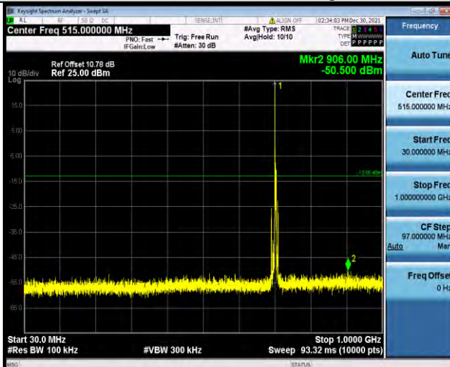
Band17-5MHz-QPSK-23790-1RB#0-Range1:30~1000MHz
