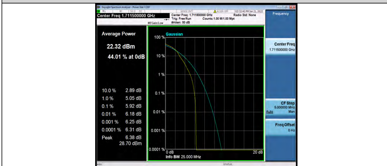
Band66-3MHz-64QAM-131987-15RB#0
