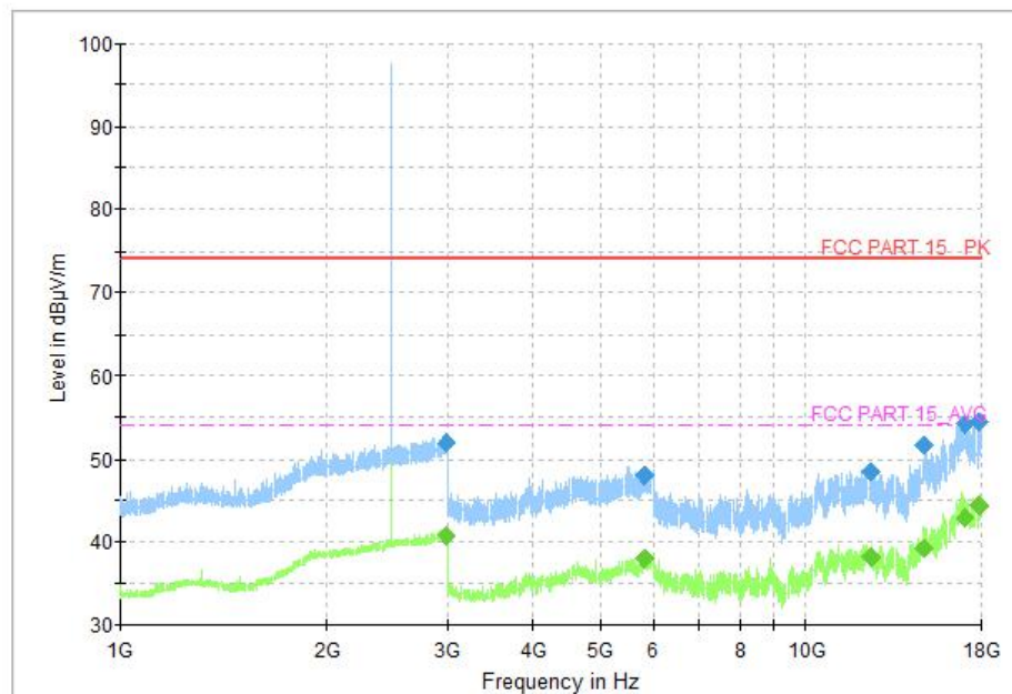
Fig.25 Radiated Spurious Emission (Ch39, 1 GHz ~18 GHz), LE 1M
