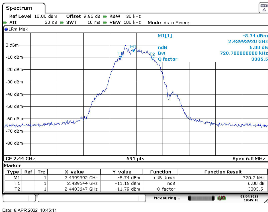
Fig.8 6dB Bandwidth (Ch 19), LE 1M
