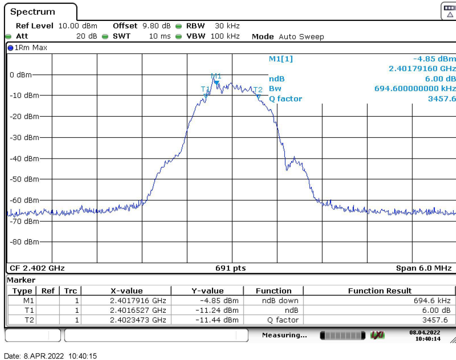
Fig.7 6dB Bandwidth (Ch 0), LE 1M
