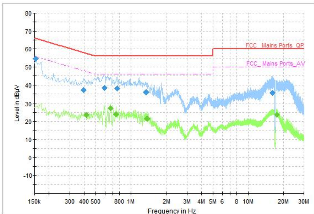
Fig.36 AC Power line Conducted Emission (Traffic), LE
