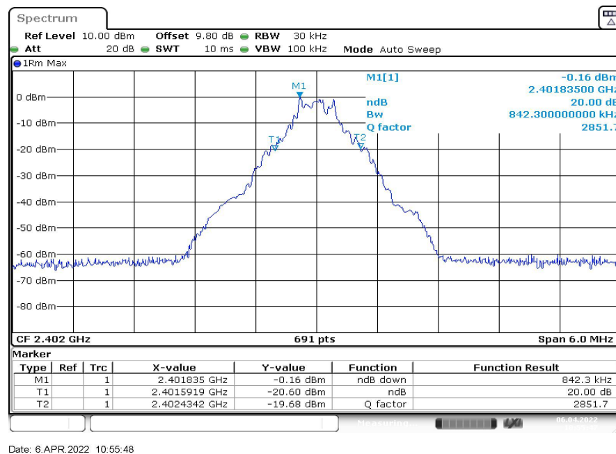
Fig. 40 20dB Bandwidth (GFSK, Ch 0)
