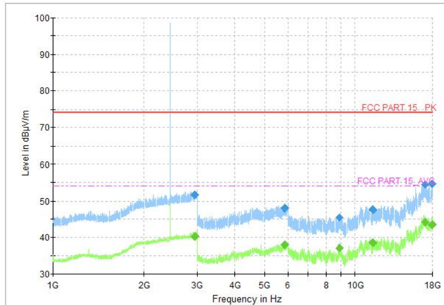
Fig. 28 Radiated Spurious Emission ( \pi/4 DQPSK, Ch39, 1 GHz ~18 GHz)
