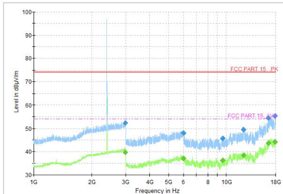
Fig. 27 Radiated Spurious Emission ( \pi/4 DQPSK, Ch0, 1 GHz ~18 GHz)
