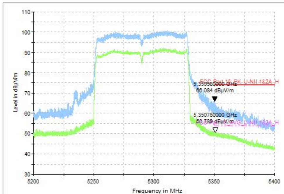
Fig. 64 Band Edges (802.11ac-VHT80, CH58 5290MHz)
