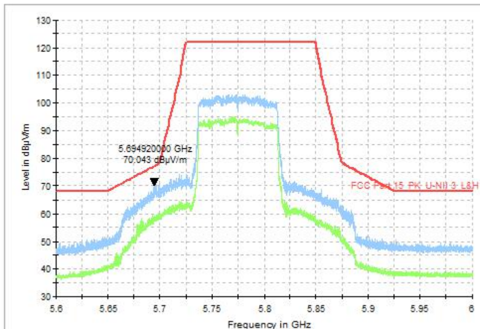
Fig. 66 Band Edges (802.11ac-VHT80, CH155 5775MHz)
