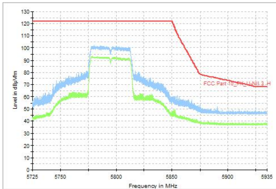
Fig. 62 Band Edges (802.11n-HT40, CH159 5795MHz)
