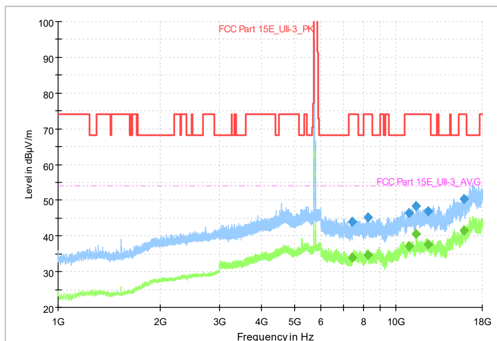
Fig. 76 Transmitter Spurious Emission (802.11a, CH149 5745MHz, 1 GHz ~18 GHz)
