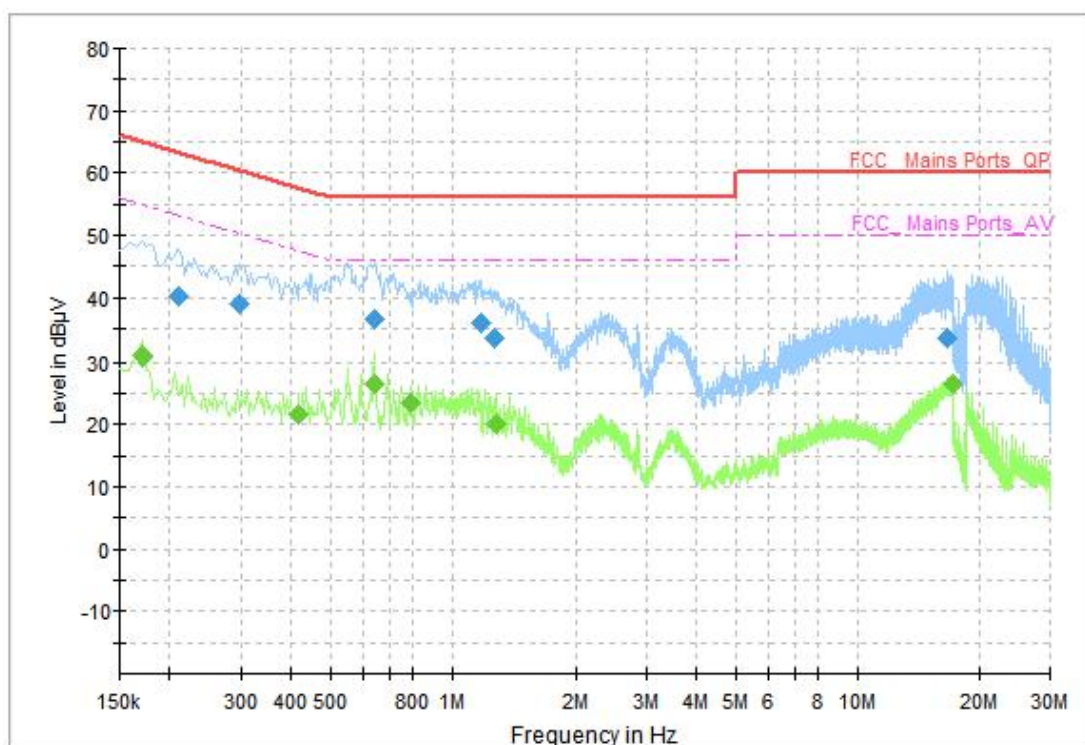
Fig. 98 AC Power line Conducted Emission (Idle)
