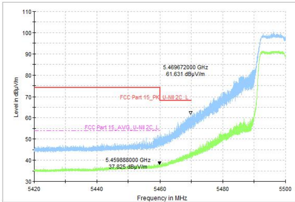
Fig. 53 Band Edges (802.11a, CH100 5500MHz)
