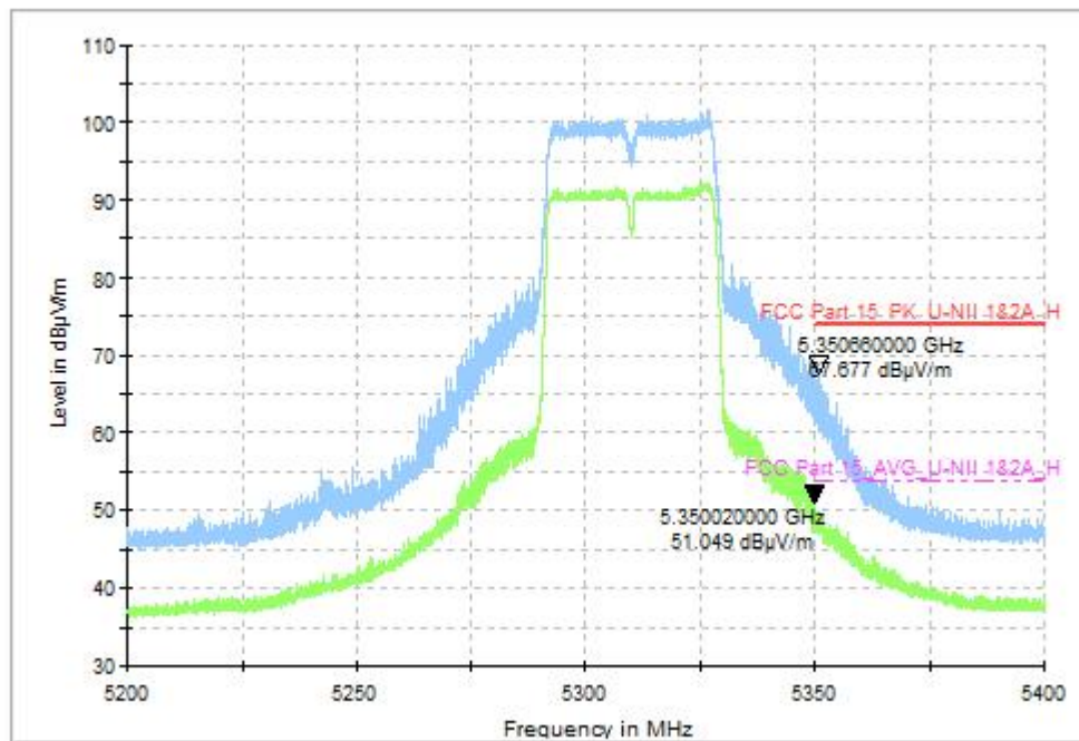
Fig. 58 Band Edges (802.11n-HT40, CH62 5310MHz)
