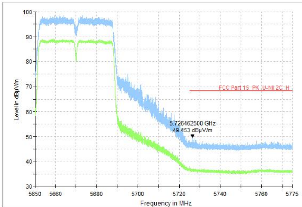
Fig. 60 Band Edges (802.11n-HT40, CH134 5670MHz)
