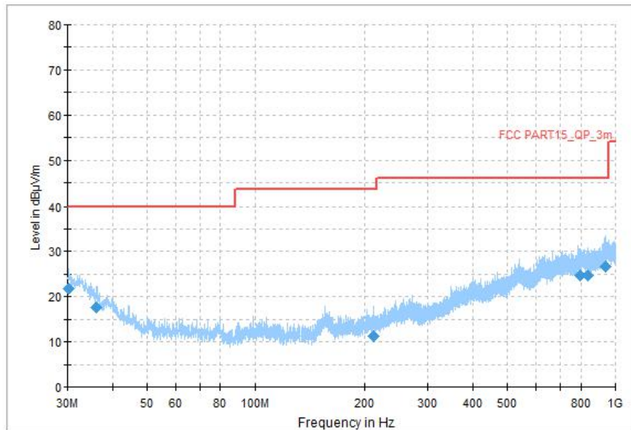
Fig. 93 Transmitter Spurious Emission (All channel, 30MHz~1GHz)
