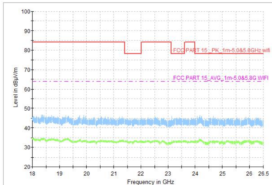
Fig. 94 Transmitter Spurious Emission (All channel, 18GHz~26.5GHz)
