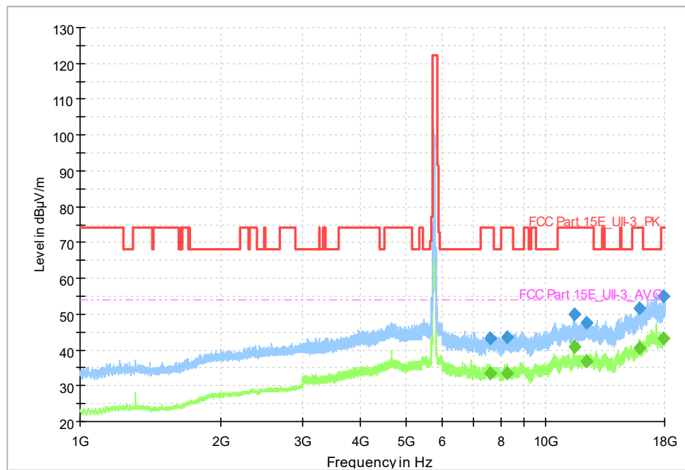
Fig. 86 Transmitter Spurious Emission (802.11n-HT40, CH151 5755MHz, 1 GHz ~18 GHz)
