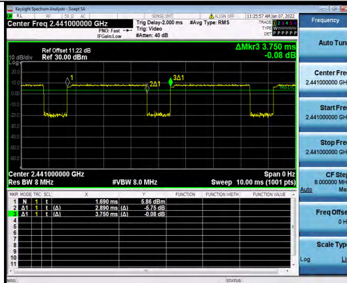
3DH5_Ant1_2441
