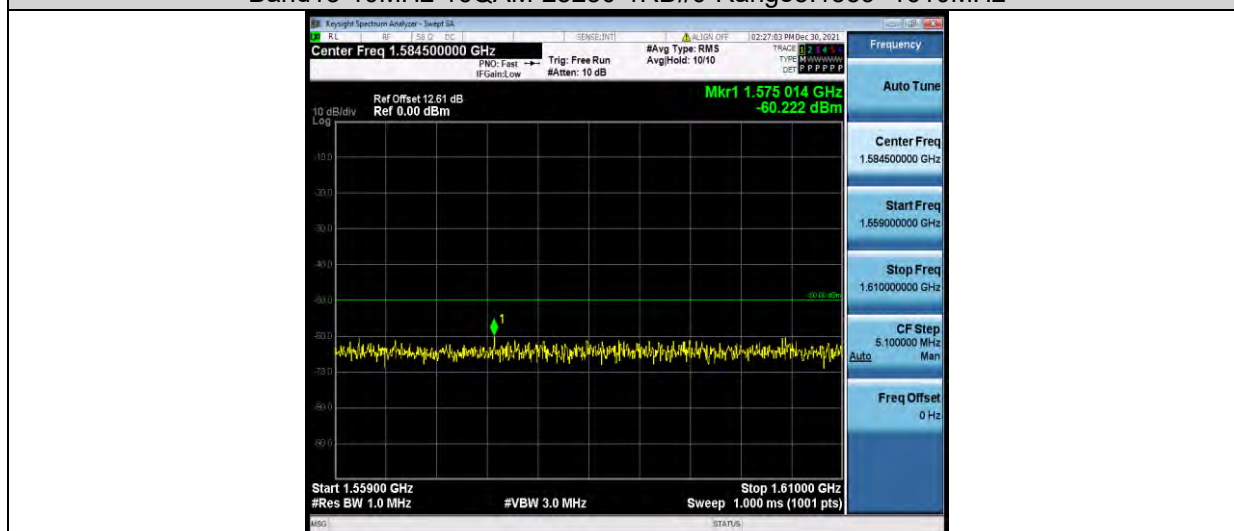
Band13-10MHz-16QAM-23230-1RB#0-Range5:1559~1610MHz
