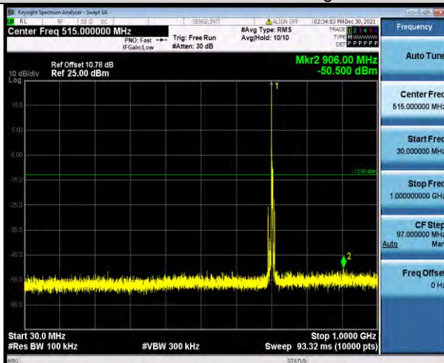
Band17-5MHz-QPSK-23790-1RB#0-Range1:30~1000MHz
