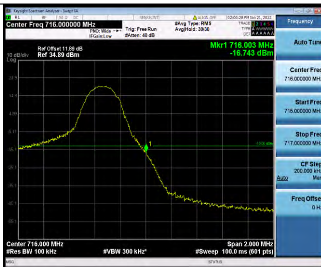
Band17-5MHz-64QAM-23825-25RB#0
