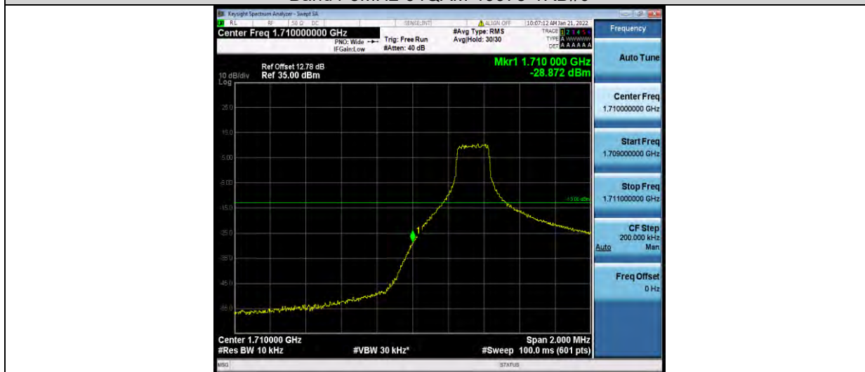
Band4-5MHz-64QAM-19975-25RB#0
