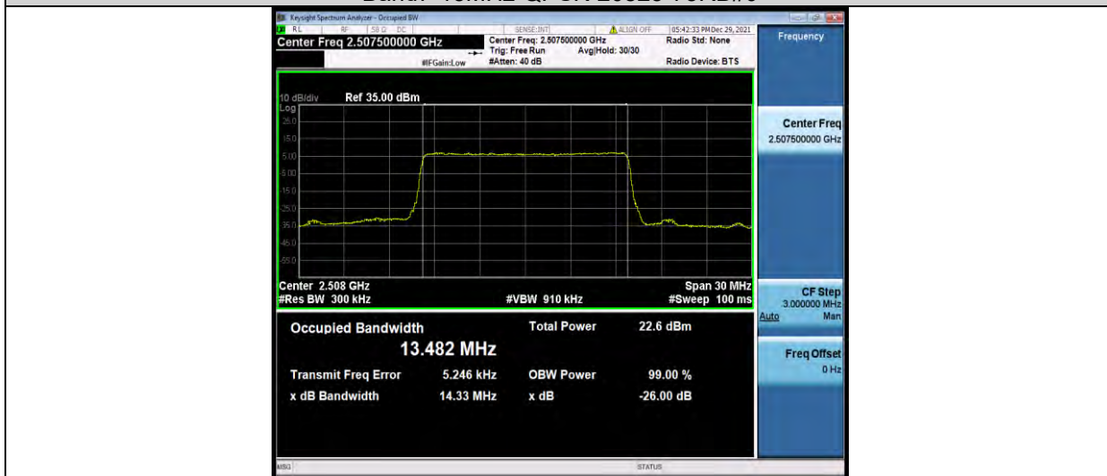
Band7-15MHz-QPSK-2100-75RB#0
