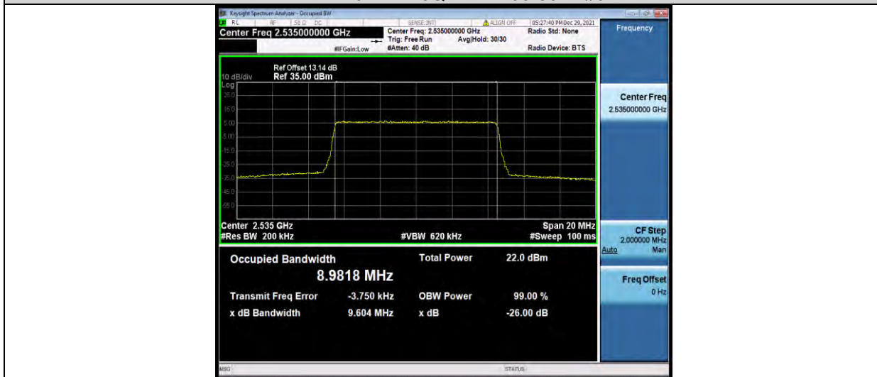
Band7-10MHz-16QAM-21400-50RB#0
