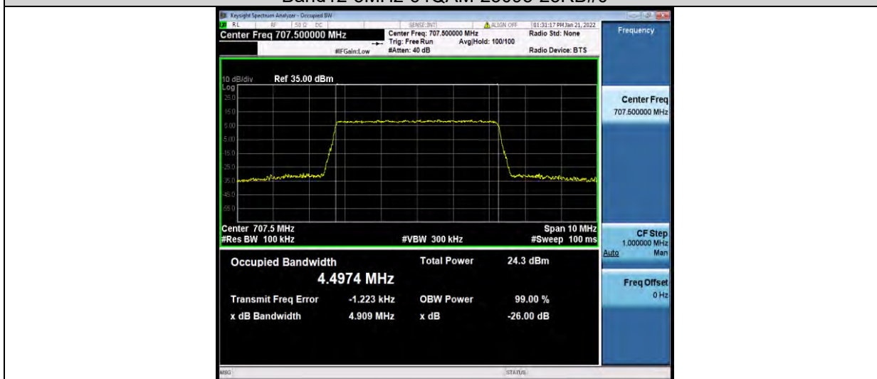
Band12-5MHz-64QAM-23155-25RB#0
