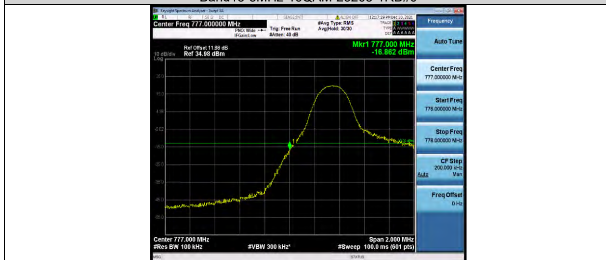
Band13-5MHz-16QAM-23205-25RB#0
