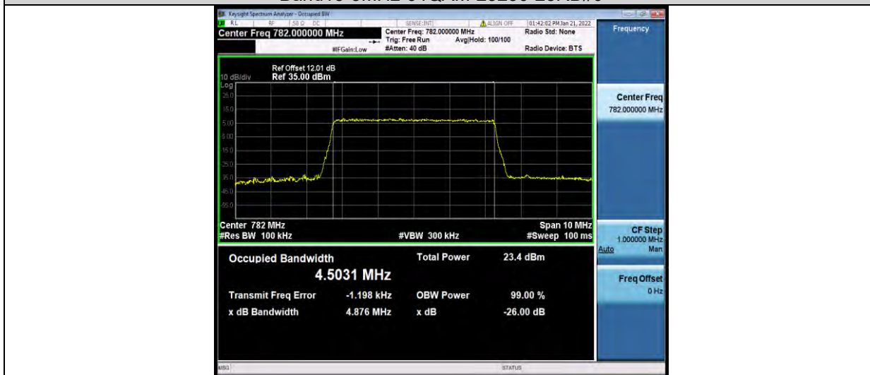
Band13-5MHz-64QAM-23255-25RB#0
