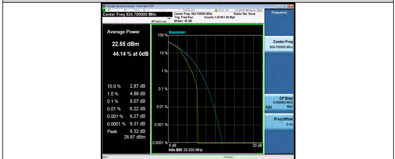
Band5-1.4MHz-64QAM-20407-6RB#0
