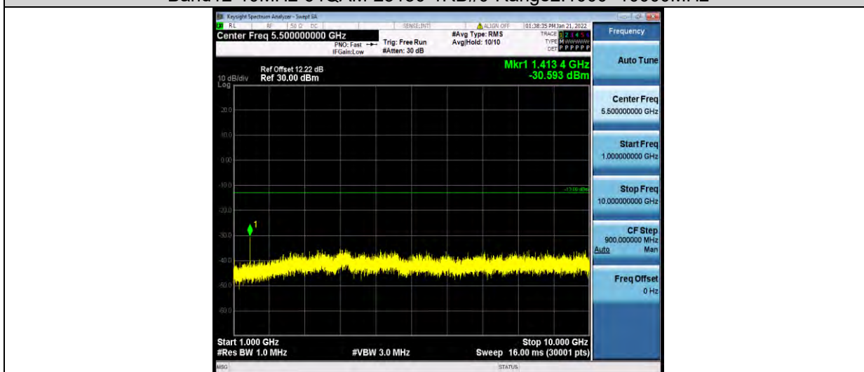
Band12-10MHz-64QAM-23130-1RB#0-Range2:1000~10000MHz
