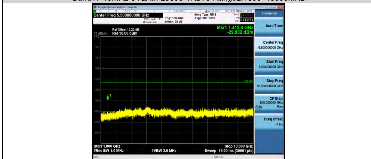
Band17-10MHz-64QAM-23800-1RB#0-Range2:1000~10000MHz
