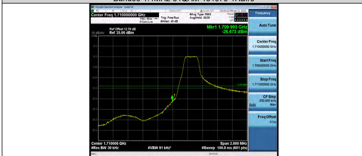
Band66-1.4MHz-64QAM-131979-6RB#0
