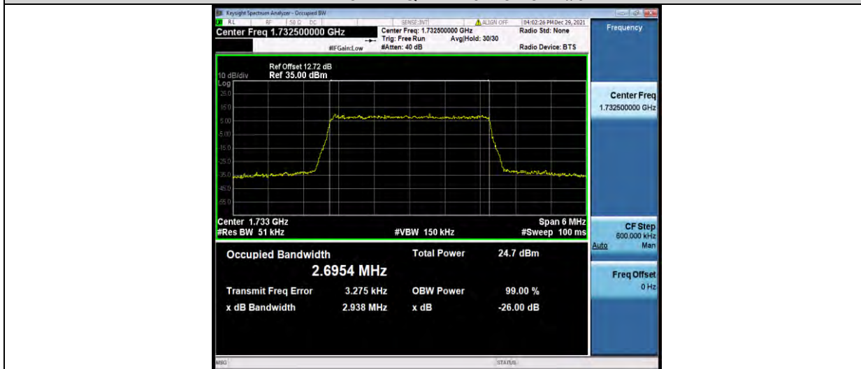
Band4-3MHz-QPSK-20385-15RB#0
