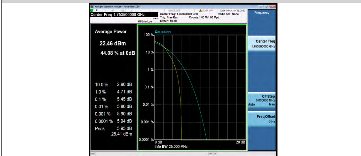
Band4-3MHz-64QAM-20385-15RB#0
