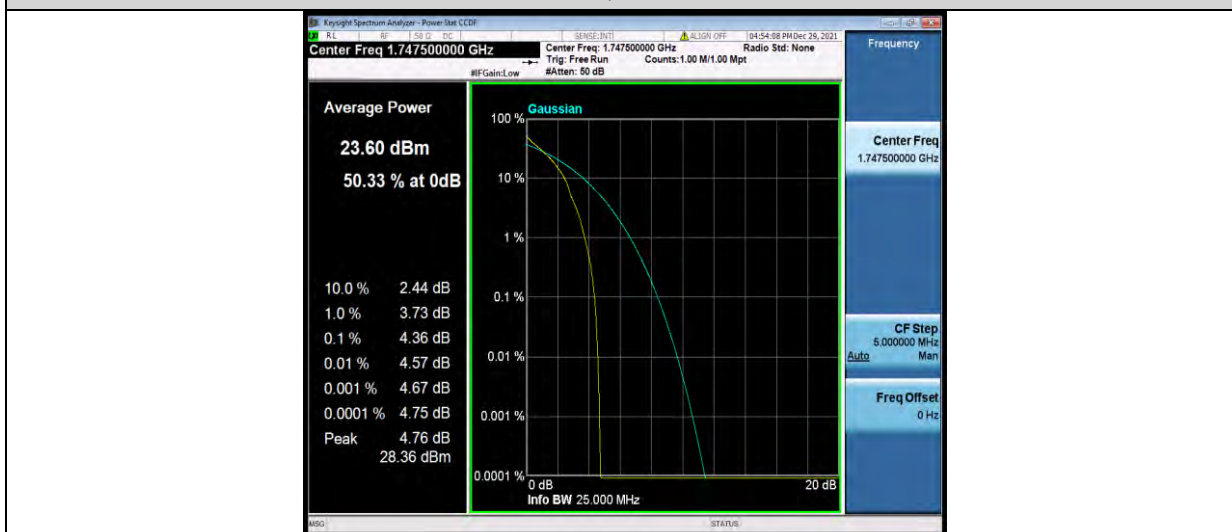
Band4-15MHz-QPSK-20325-75RB#0
