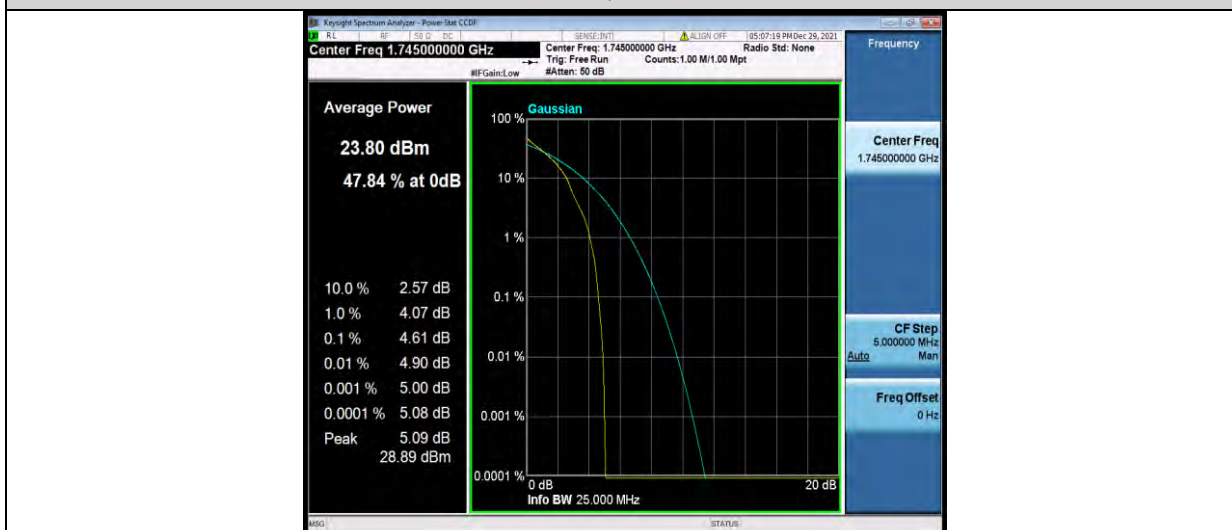
Band4-20MHz-QPSK-20300-100RB#0
