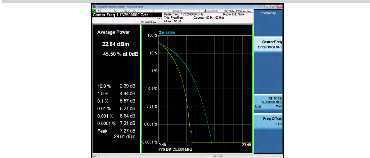
Band4-20MHz-QPSK-20300-1RB#0
