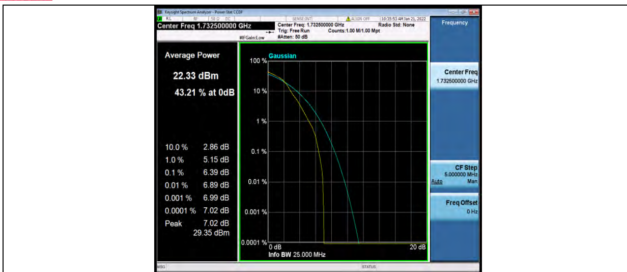
Band4-3MHz-64QAM-20175-15RB#0
