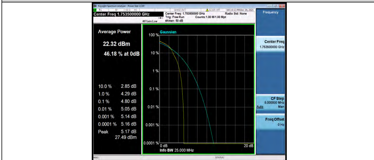
Band4-3MHz-16QAM-20385-15RB#0
