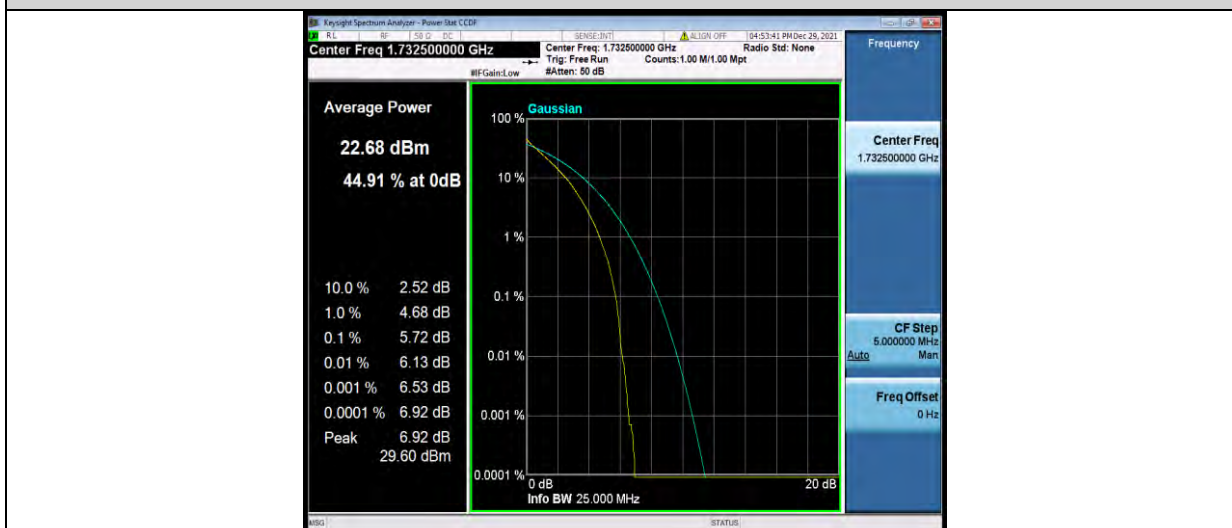
Band4-15MHz-QPSK-20325-1RB#0
