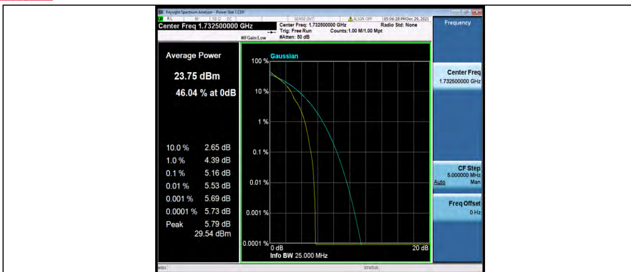
Band4-20MHz-QPSK-20175-100RB#0
