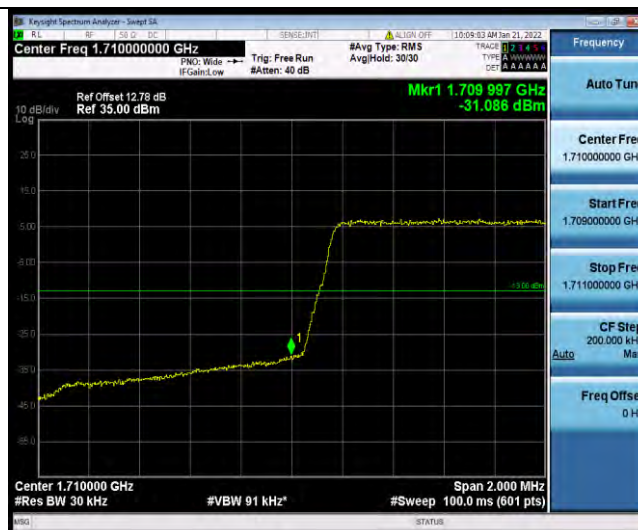
Band4-1.4MHz-64QAM-20350-1RB#5
