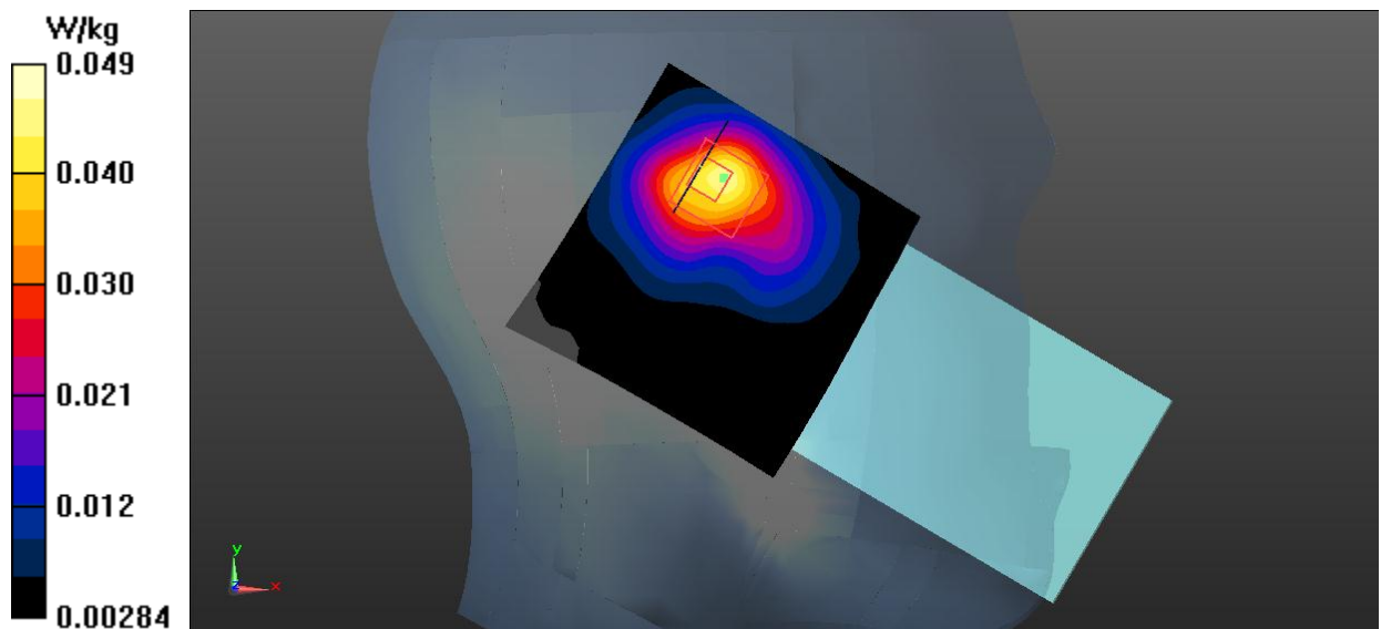
Fig.23 Bluetooth Head
