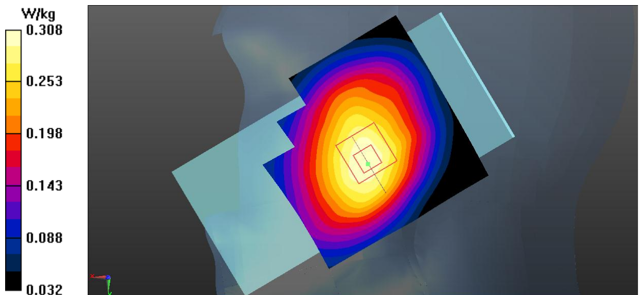
Fig.1 GSM850 Head
