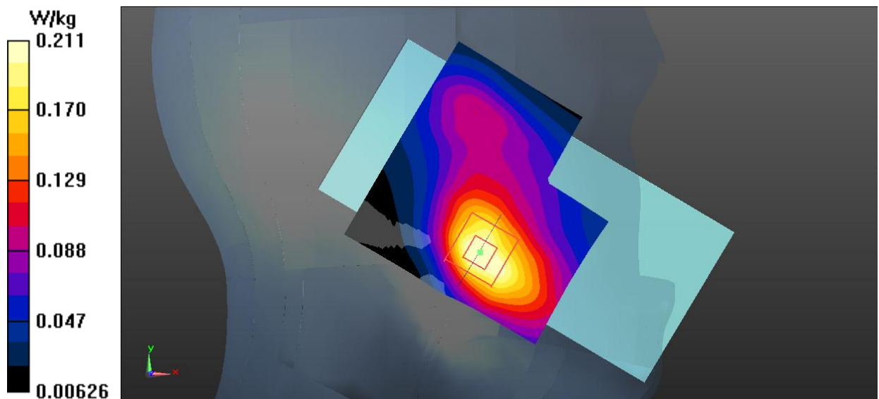
Fig.3 GSM1900 Head
