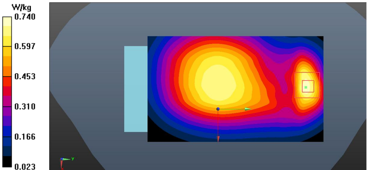
Fig.2 GSM850 Body
