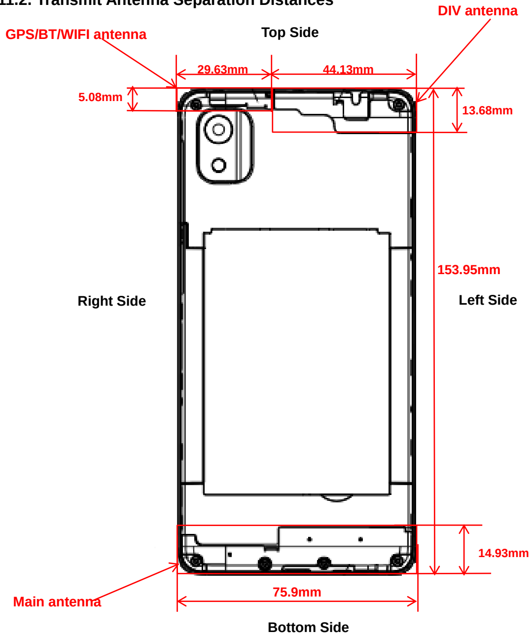
Picture 11.1 Antenna Locations (Back view)
