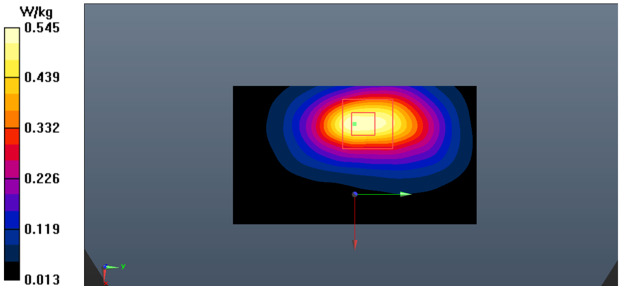
Fig.4 GSM1900 Body
