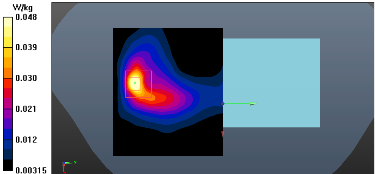
Fig.24 Bluetooth Body
