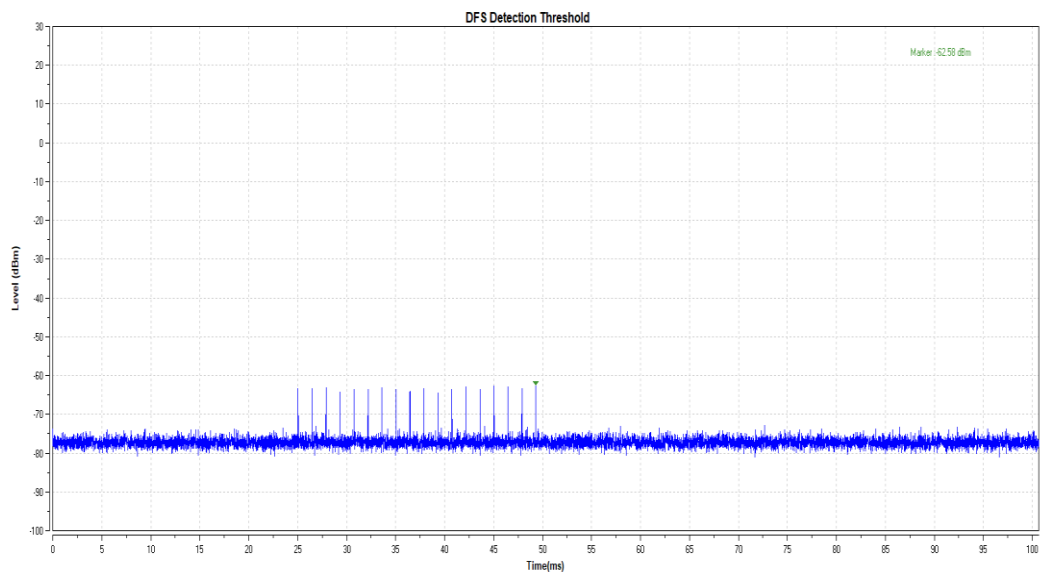
11N40SISO_5270_Type0
