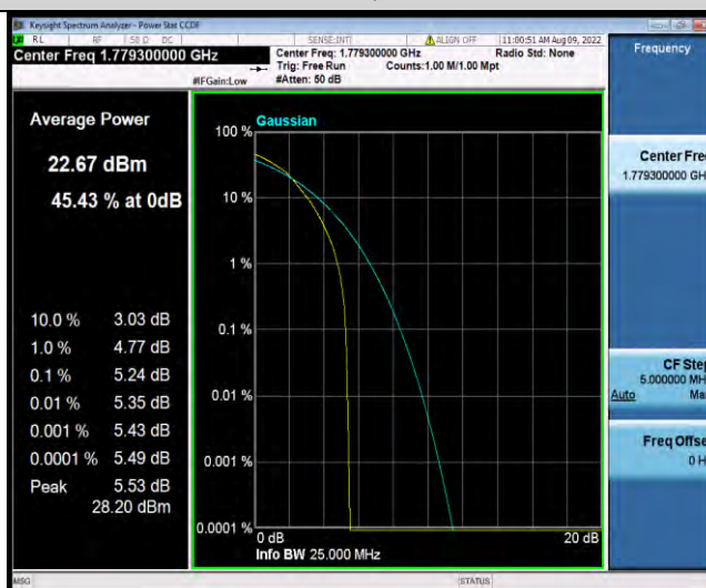
Band66-1.4MHz-64QAM-132665-6RB#0
