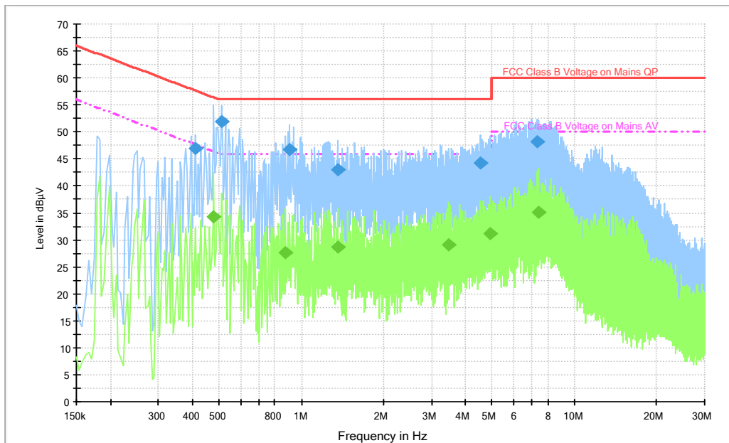
Fig A.19 Conducted Emission
