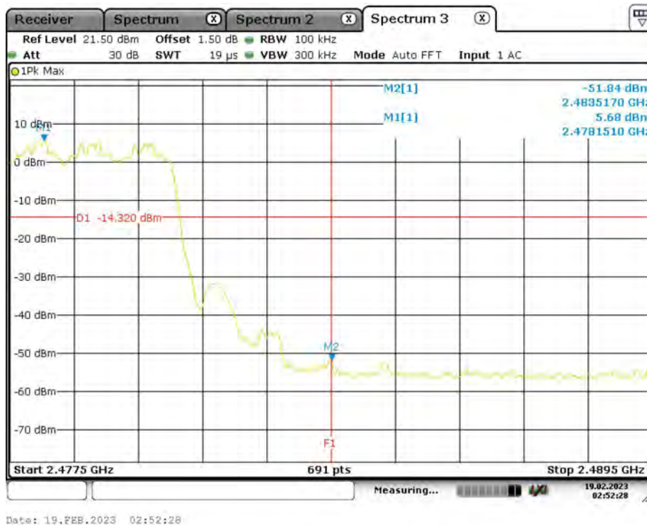
2DH5_Ant1_High_Hop_2480
