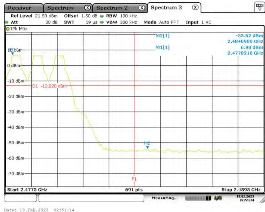
DH5_Ant1_High_Hop_2480
