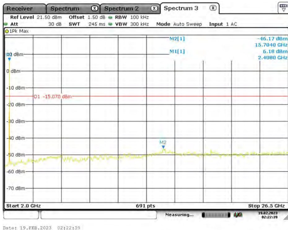
3DH5_Ant1_2402_2000~26500
