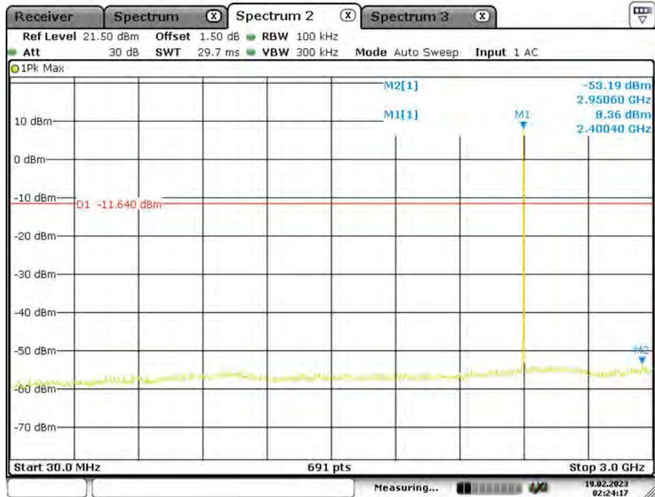
3DH5_Ant1_2402_30~3000
