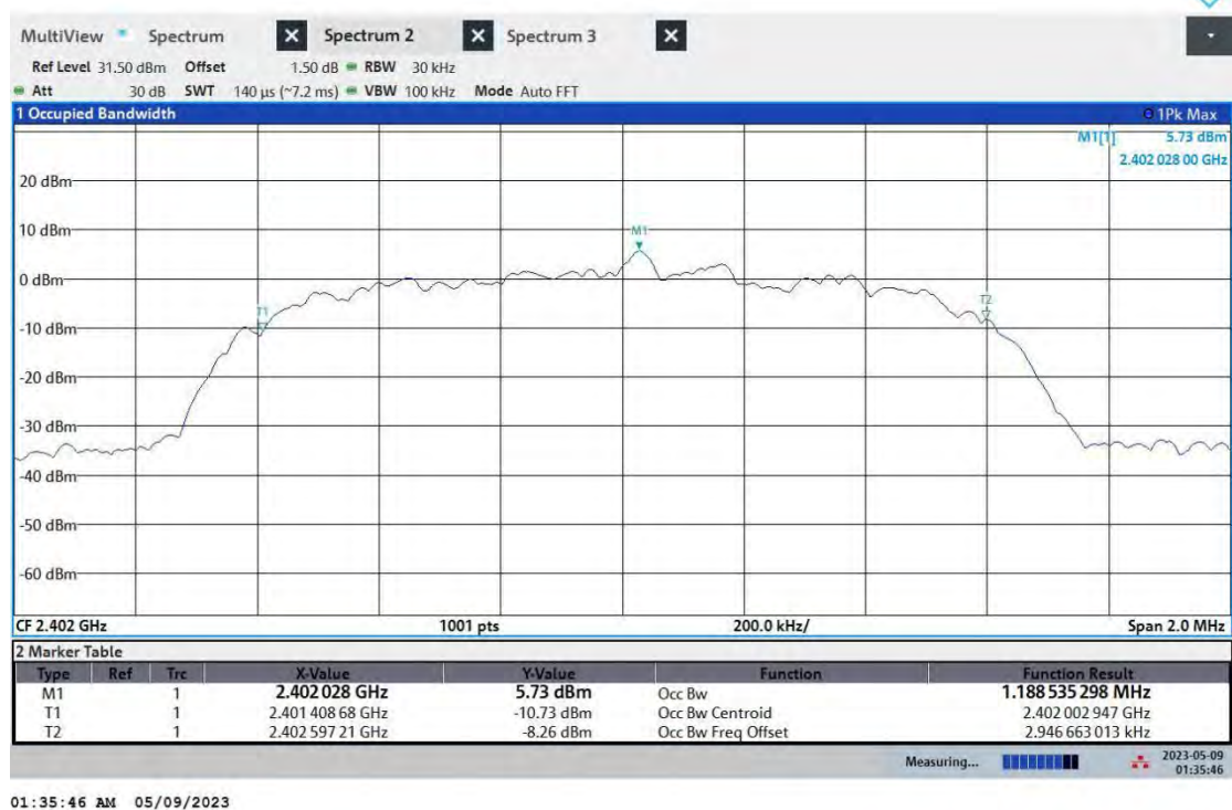
3DH5_Ant1_2402
