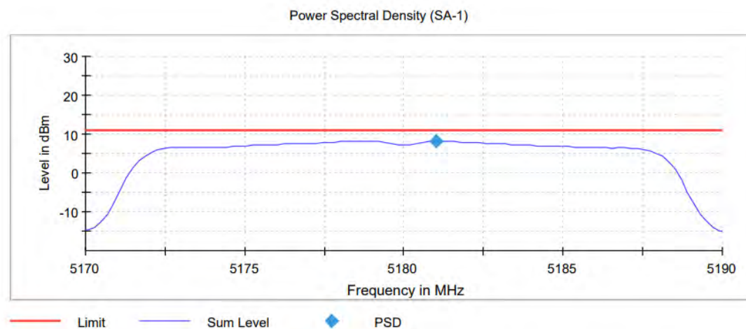
11A_An0_5180
