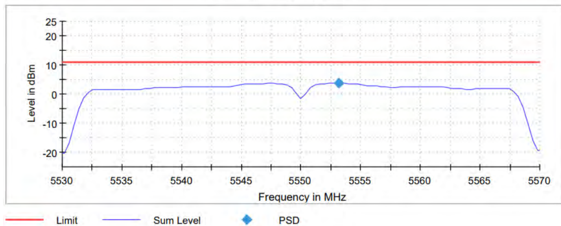
Power Spectral Density (SA-1)
