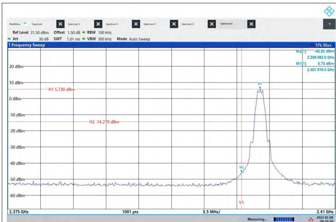
BLE_1M_Ant1_Low_2402
