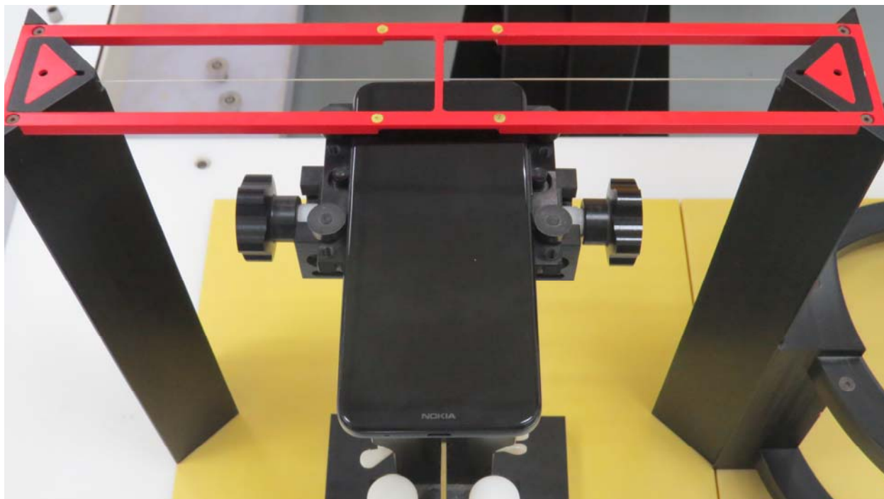
Picture 1: HAC Test setup
