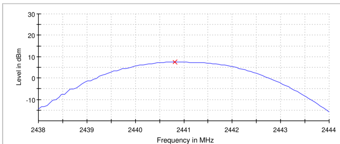
Peak Power
