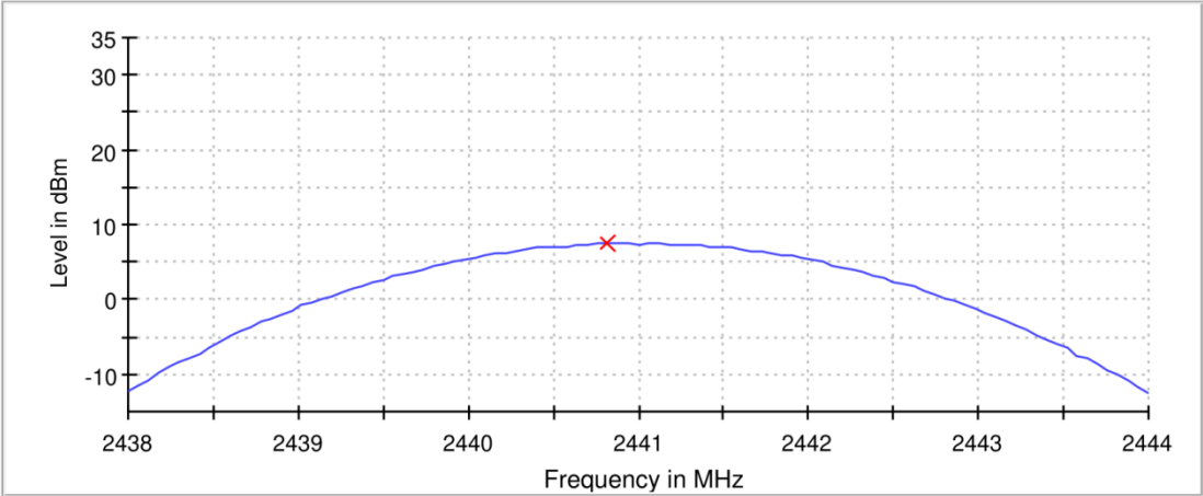
Peak Power
