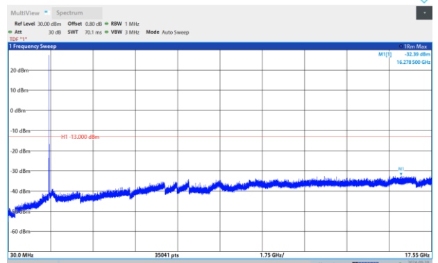
Band4-5MHz-16QAM-20375-1RB#0-Range:30~17550M Hz
