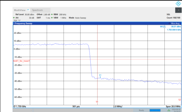
Band4-20MHz-16QAM-20050-100RB#0
