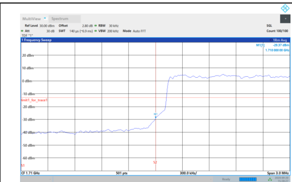
Band4-3MHz-QPSK-20385-15RB#0
