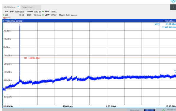
Band4-10MHz-QPSK-20000-1RB#0-Range:30~17550 MHz
