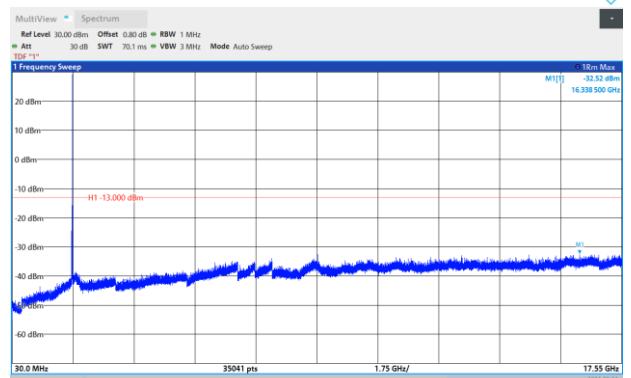
Band4-10MHz-QPSK-20175-1RB#0-Range:30~17550M Hz
