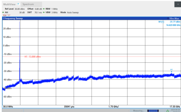
Band4-15MHz-QPSK-20325-1RB#0-Range:30~17550 MHz
