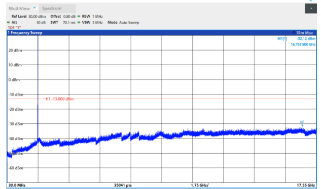
Band4-5MHz-QPSK-20175-1RB#0-Range:30~17550MHz Z
