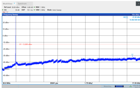
Band4-10MHz-QPSK-20350-1RB#0-Range:30~17550 MHz
