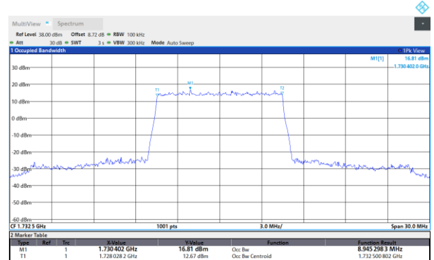
Band4-10MHz-16QAM-20000-50RB#0
