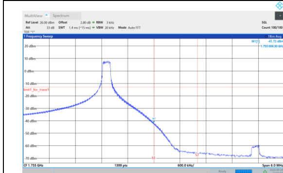
Band4-20MHz-16QAM-20300-1RB#99
