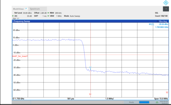
Band4-15MHz-16QAM-20025-75RB#0
