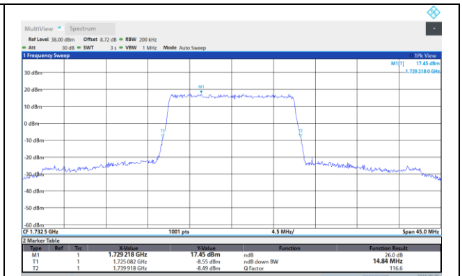
Band4-15MHz-16QAM-20025-75RB#0
