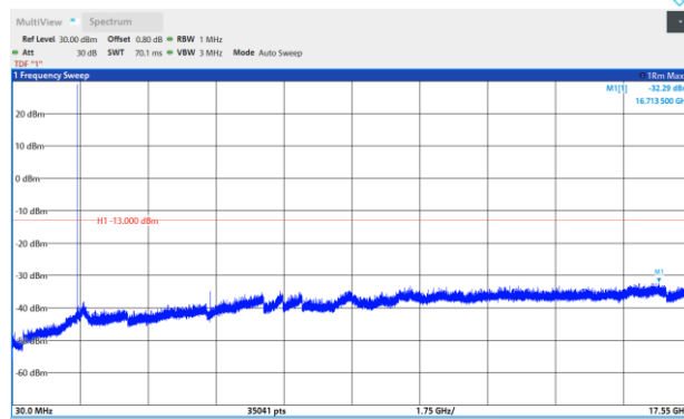
Band4-1.4MHz-16QAM-20393-1RB#0-Range:30~17550 MHz
