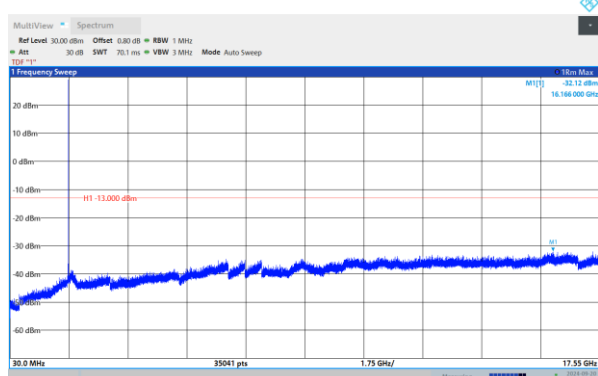
Band4-1.4MHz-16QAM-20175-1RB#0-Range:30~175 50MHz
