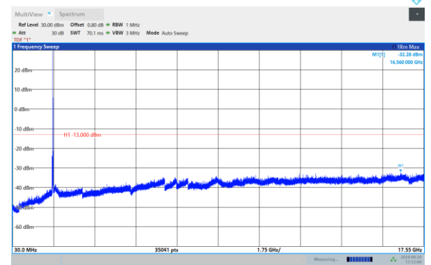
Band4-15MHz-16QAM-20175-1RB#0-Range:30~17550 MHz
