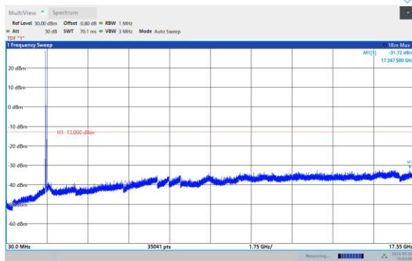
Band4-20MHz-QPSK-20300-1RB#0-Range:30~17550 MHz
