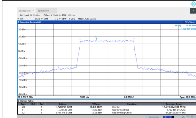
Band4-20MHz-16QAM-20175-100RB#0
