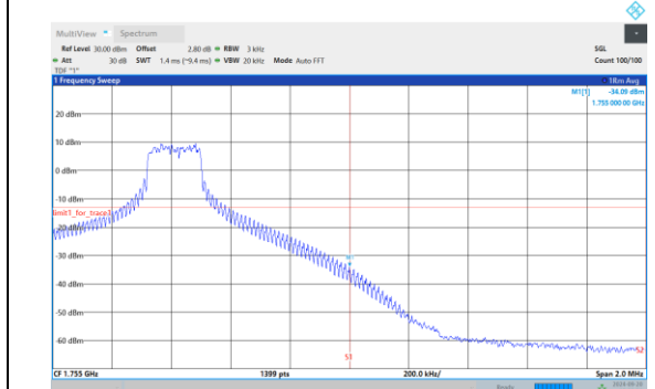
Band4-10MHz-16QAM-20000-1RB#0
