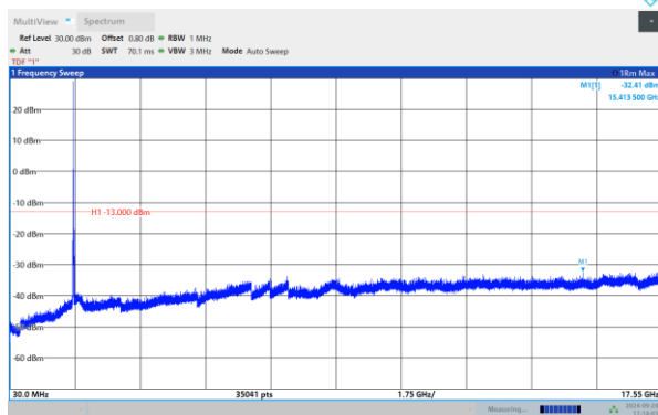
Band4-20MHz-16QAM-20175-1RB#0-Range:30~17550 OMHz
