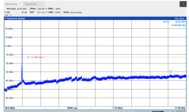
Band4-20MHz-16QAM-20300-1RB#0-Range:30~17550 MHz
