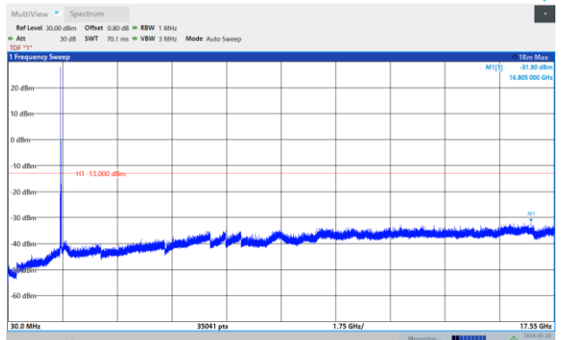
Band4-15MHz-16QAM-20325-1RB#0-Range:30~17550 MHz
