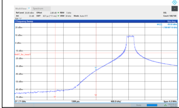
Band4-15MHz-16QAM-20325-1RB#74
