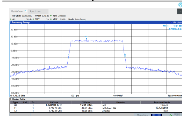
Band4-20MHz-16QAM-20175-100RB#0
