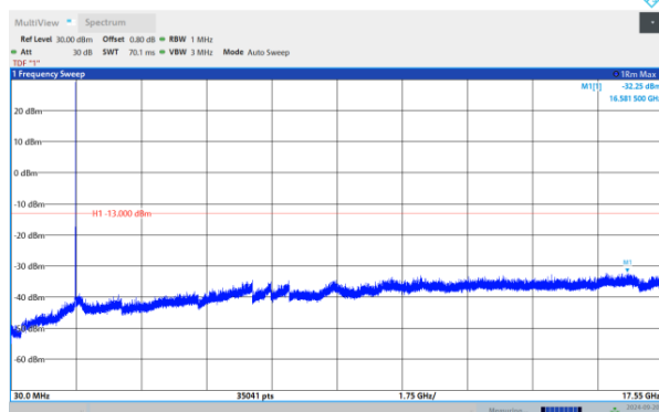
Band4-3MHz-16QAM-20175-1RB#0-Range:30~17550 MHz
