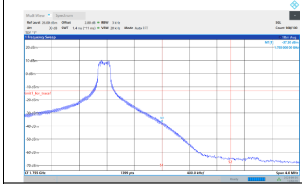
Band4-15MHz-16QAM-20025-1RB#0
