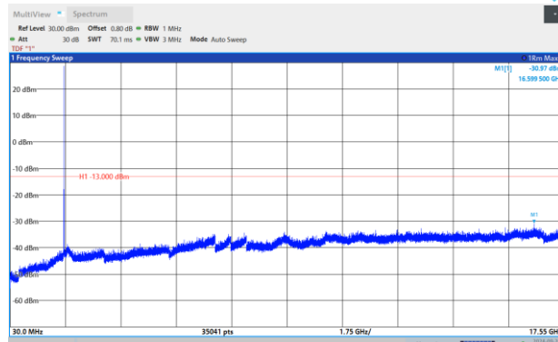
Band4-1.4MHz-16QAM-19957-1RB#0-Range:30~17550 MHz
