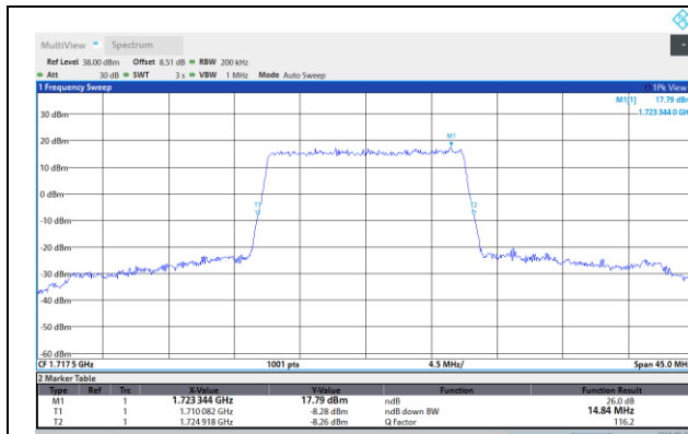
Band4-15MHz-QPSK-20175-75RB#0
