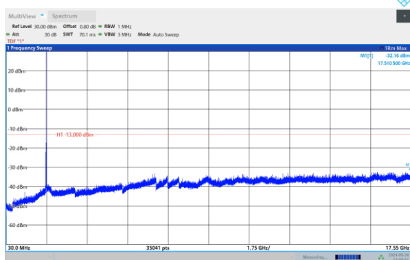
Band4-5MHz-16QAM-20175-1RB#0-Range:30~17550 MHz
