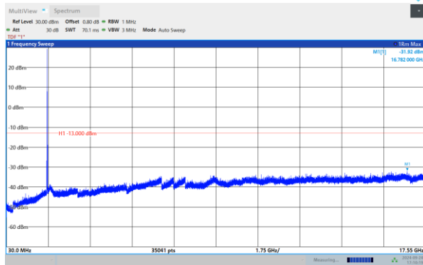
Band4-15MHz-QPSK-20025-1RB#0-Range:30~17550 MHz
