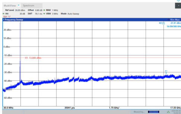
Band4-5MHz-QPSK-20375-1RB#0-Range:30~17550 MHz
