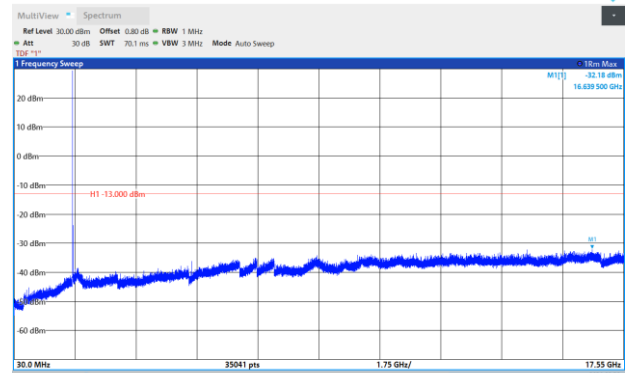
Band4-3MHz-16QAM-20385-1RB#0-Range:30~17550M Hz
