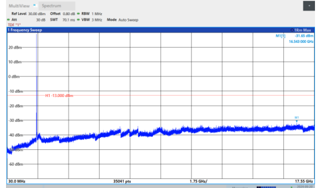
Band4-10MHz-16QAM-20350-1RB#0-Range:30~17550 MHz
