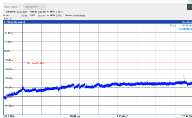
Band4-3MHz-QPSK-20175-1RB#0-Range:30~17550MH Z
