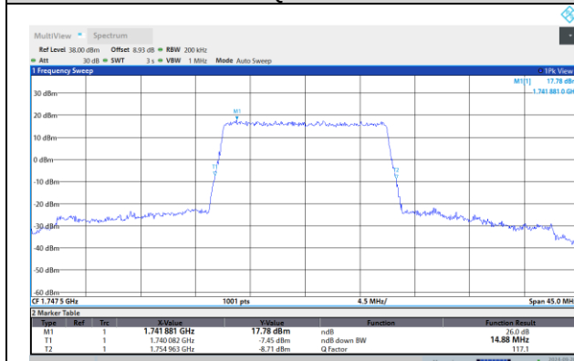
Band4-15MHz-16QAM-20175-75RB#0
