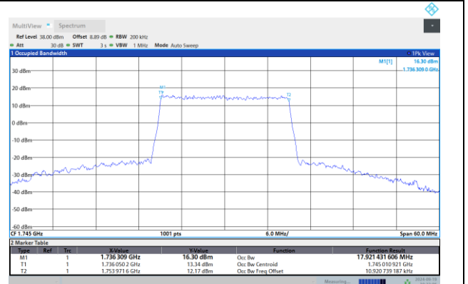
Band4-20MHz-16QAM-20300-100RB#0
