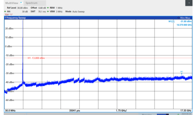
Band4-10MHz-16QAM-20000-1RB#0-Range:30~17550 MHz
