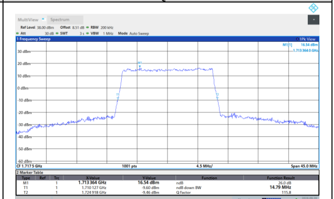
Band4-15MHz-16QAM-20325-75RB#0
