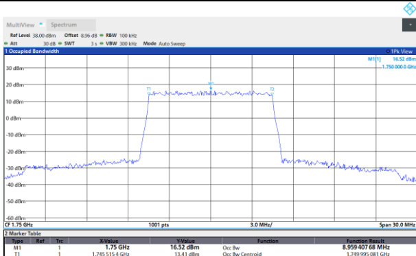
Band4-10MHz-16QAM-20175-50RB#0
