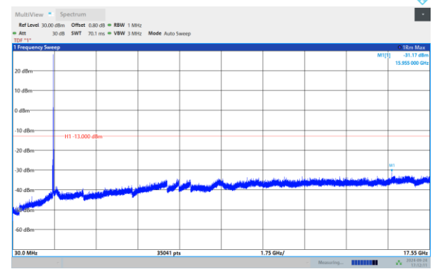
Band4-20MHz-QPSK-20050-1RB#0-Range:30~17550 MHz
