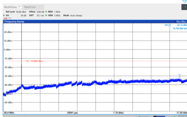
Band4-5MHz-QPSK-19975-1RB#0-Range:30~17550 MHz
