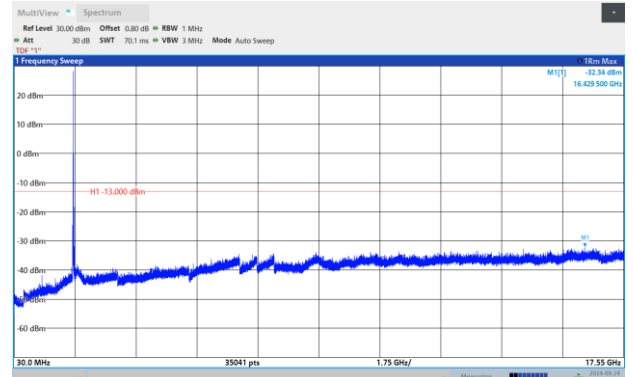
Band4-20MHz-16QAM-C-1RB#0-Range:30~17550MHz
