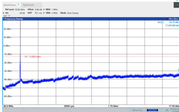
Band4-10MHz-16QAM-20175-1RB#0-Range:30~17550 MHz
