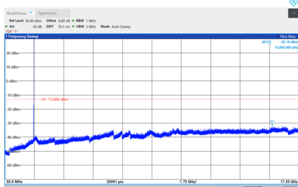
Band4-3MHz-QPSK-19965-1RB#0-Range:30~17550 MHz
