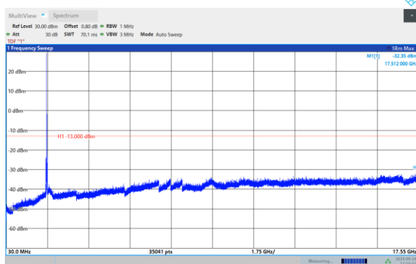
Band4-20MHz-16QAM-20175-1RB#0-Range:30~17550 OMHz
