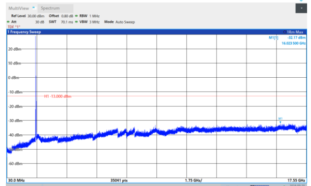
Band4-20MHz-16QAM-20300-1RB#0-Range:30~17550 MHz
