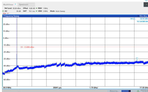
Band4-3MHz-QPSK-20385-1RB#0-Range:30~17550 MHz
