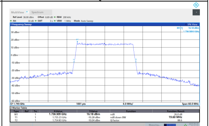
Band4-20MHz-16QAM-20300-100RB#0
