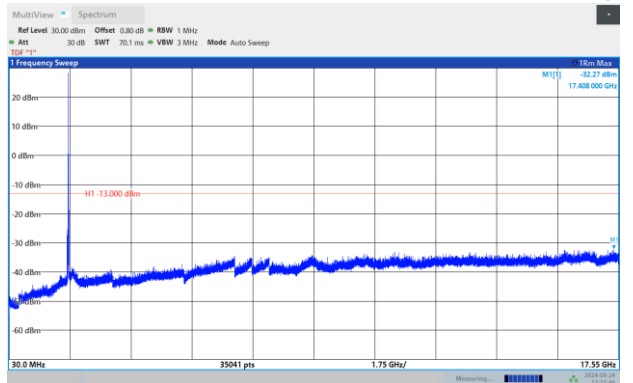
Band4-15MHz-16QAM-20025-1RB#0-Range:30~17550 MHz
