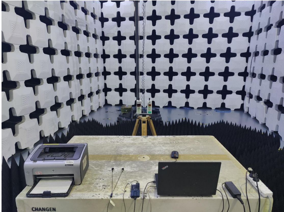
6. Radiated Emissions (Part 15B Data transfer, 18GHz-26.5GHz)
