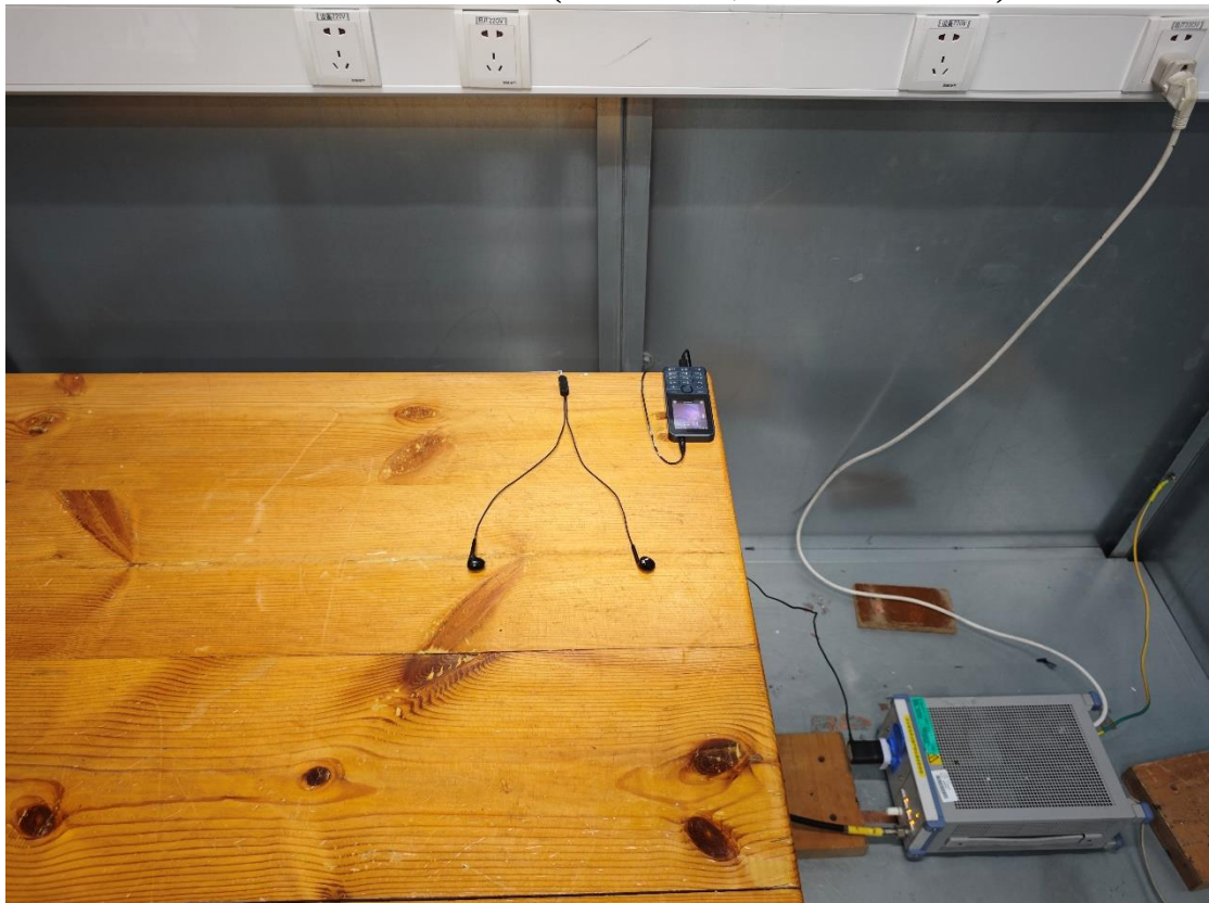
13. Conducted Emission (Part 15B, GSM receiver/WCDMA receiver /LTE)
