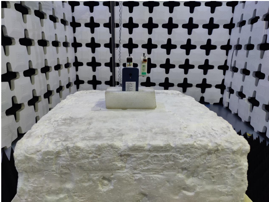
12. Radiated Emissions (Par22/24/27, 18GHz -26.5GHz)
