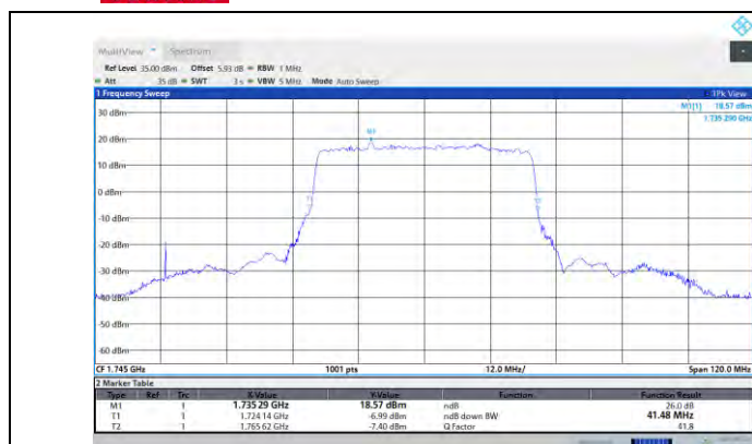
N66-PC3-40MHz-M-DFT-PI2BPSK-Outer_Full
