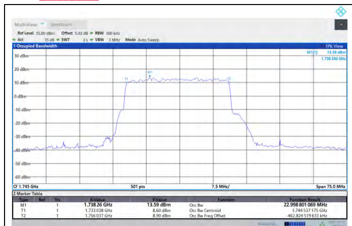
N66-PC3-25MHz-M-DFT-256QAM-Outer_Full
