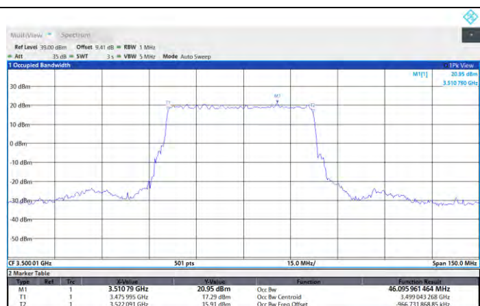
N77-3450-3550-PC2-30-50-M-DFT-PI2BPSK-Outer_Full
