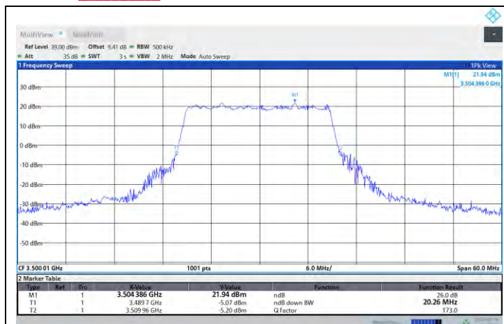
N77-3450-3550-PC2-30-20-M-DFT-PI2BPSK-Outer_Full
