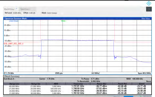
N66-PC3-40MHz-H-DFT-QPSK-Outer Full
