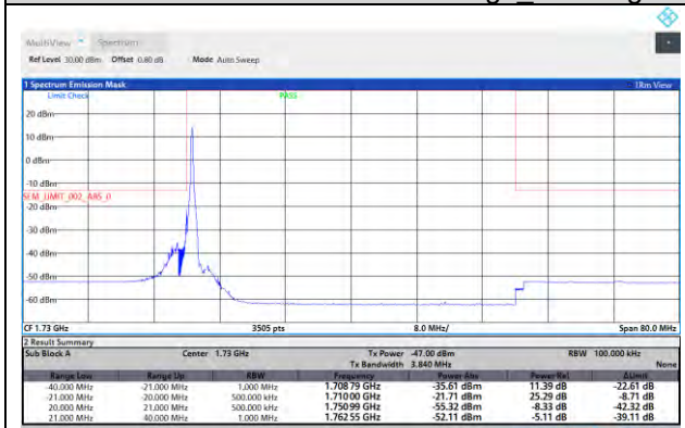
N66-PC3-40MHz-L-DFT-QPSK-Edge 1RB Left
