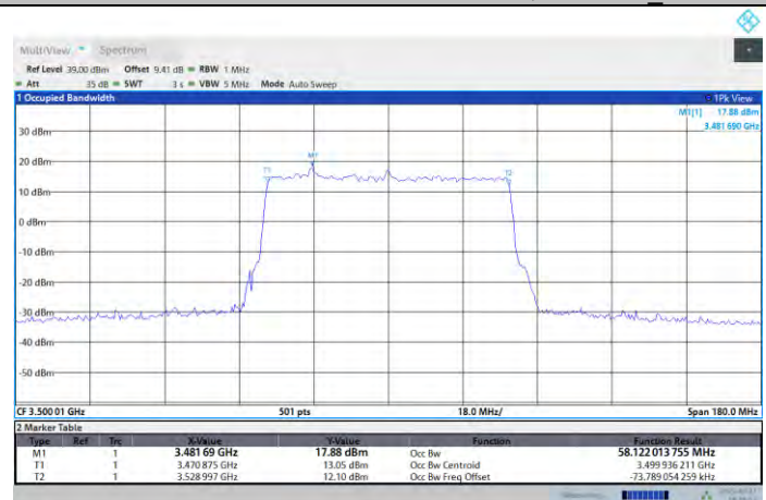
N77-3450-3550-PC2-30-60-M-DFT-256QAM-Outer_Full
