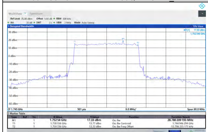
N66-PC3-30MHz-M-DFT-QPSK-Outer_Full
