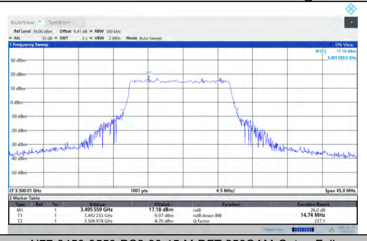
N77-3450-3550-PC2-30-15-M-DFT-256QAM-Outer_Full
