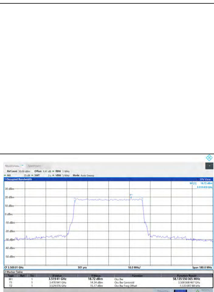
N77-3450-3550-PC2-30-60-M-DFT-16QAM-Outer_Full
