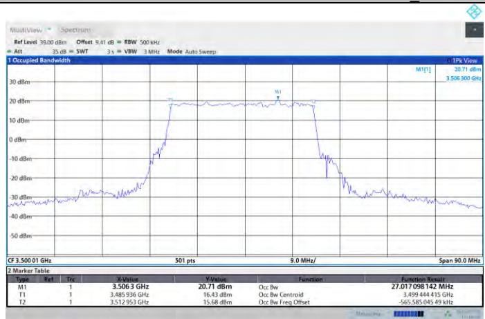
N77-3450-3550-PC2-30-30-M-DFT-PI2BPSK-Outer_Full
