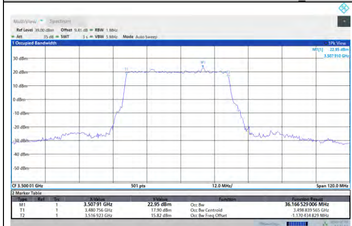
N77-3450-3550-PC2-30-40-M-DFT-PI2BPSK-Outer_Full
