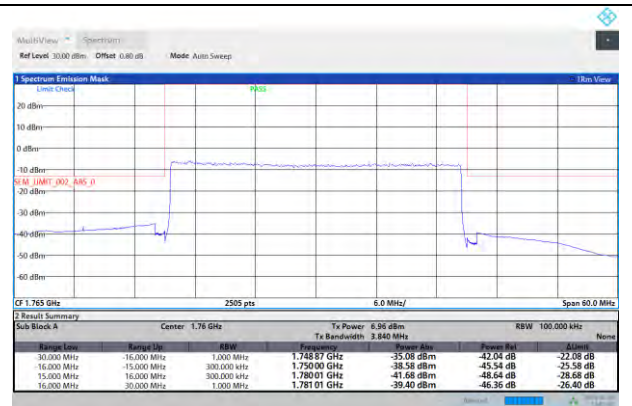
N66-PC3-30MHz-H-DFT-QPSK-Outer Full
