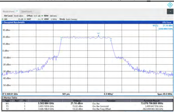
N77-3450-3550-PC2-30-15-M-DFT-PI2BPSK-Outer_Full
