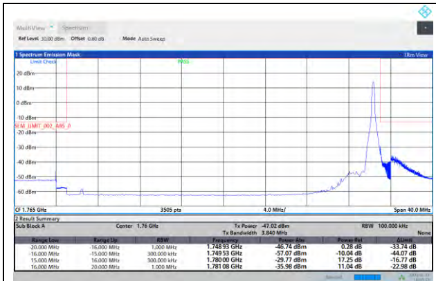
N66-PC3-30MHz-H-DFT-QPSK-Edge 1RB-Right
