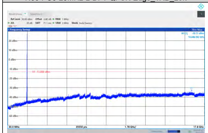
N66-PC3-25MHz-H-DFT-QPSK-Edge_1RB_Left
