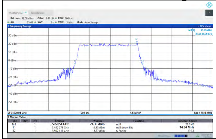
N77-3450-3550-PC2-30-15-M-DFT-QPSK-Outer_Full
