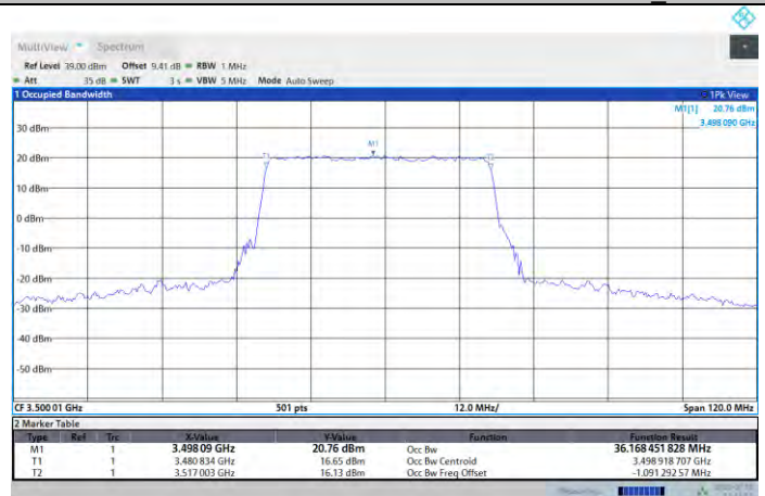
N77-3450-3550-PC2-30-40-M-DFT-QPSK-Outer_Full
