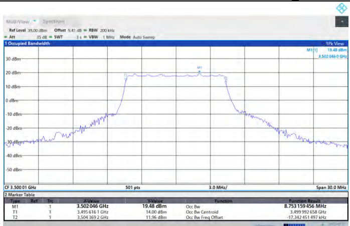
N77-3450-3550-PC2-30-10-M-DFT-64QAM-Outer_Full
