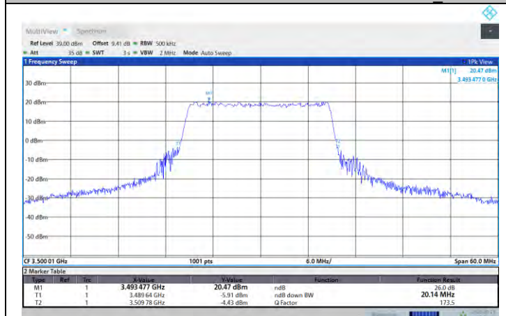
N77-3450-3550-PC2-30-20-M-DFT-16QAM-Outer_Full
