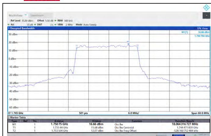
N66-PC3-20MHz-M-DFT-64QAM-Outer_Full
