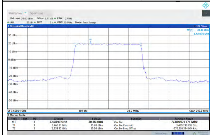
N77-3450-3550-PC2-30-80-M-DFT-64QAM-Outer_Full
