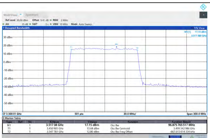
N77-3450-3550-PC2-30-100-M-DFT-256QAM-Outer_Full
