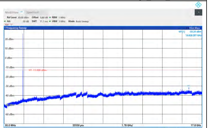
N66-PC3-10MHz-L-DFT-QPSK-Edge_1RB_Left
