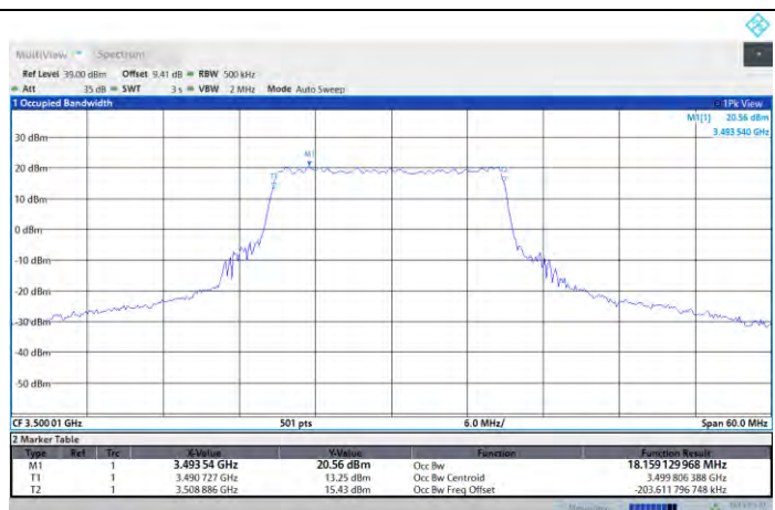
N77-3450-3550-PC2-30-20-M-DFT-64QAM-Outer_Full
