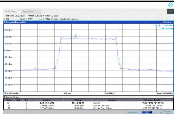
N77-3450-3550-PC2-30-80-M-DFT-256QAM-Outer_Full
