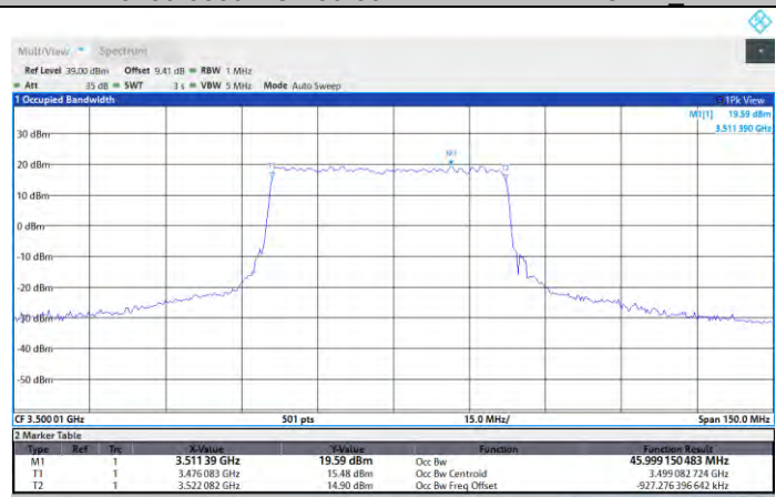
N77-3450-3550-PC2-30-50-M-DFT-16QAM-Outer_Full
