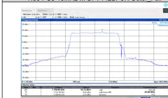
N66-PC3-40MHz-M-DFT-16QAM-Outer_Full
