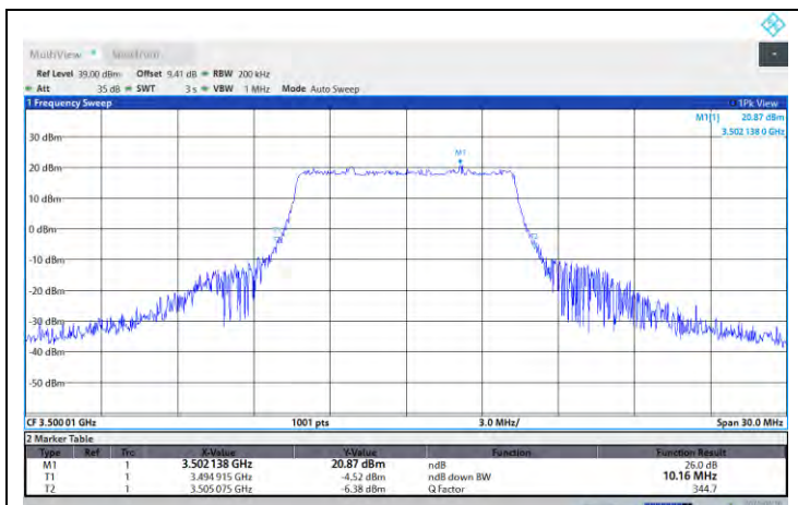
N77-3450-3550-PC2-30-10-M-DFT-PI2BPSK-Outer_Full
