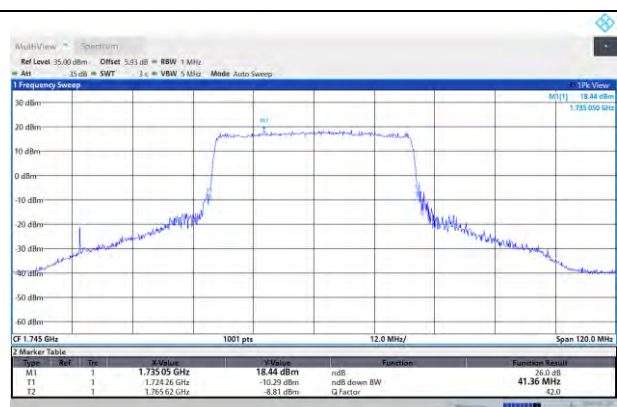
N66-PC3-40MHz-M-DFT-QPSK-Outer_Full
