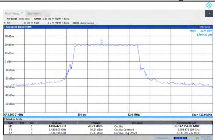
N77-3450-3550-PC2-30-40-M-DFT-64QAM-Outer_Full
