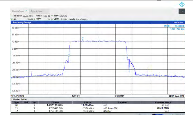
N66-PC3-30MHz-M-DFT-256QAM-Outer_Full
