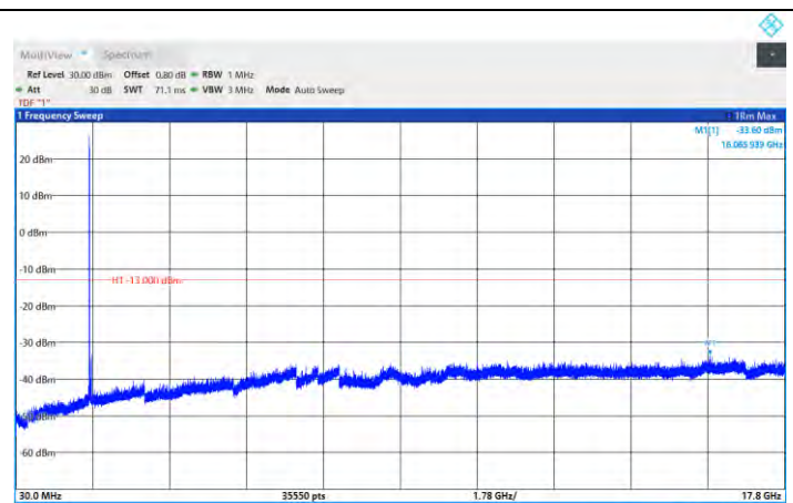
N66-PC3-40MHz-M-DFT-QPSK-Edge_1RB_Left
