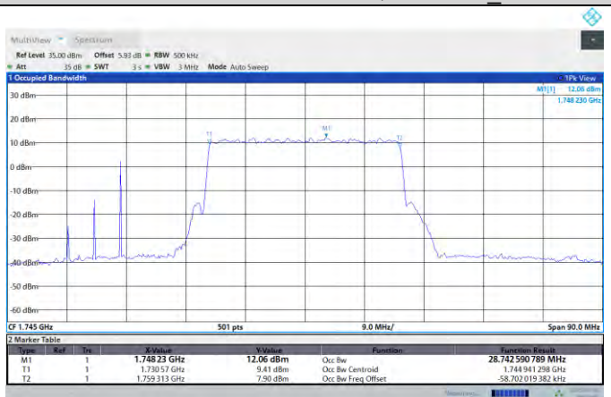
N66-PC3-30MHz-M-DFT-256QAM-Outer_Full
