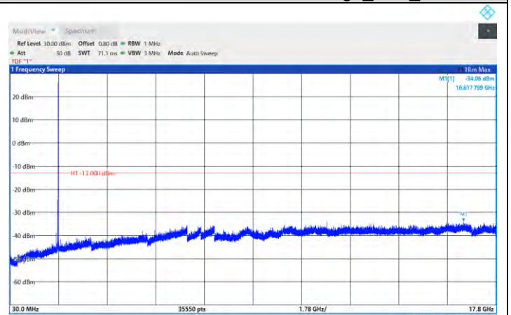
N66-PC3-10MHz-H-DFT-QPSK-Edge_1RB_Left
