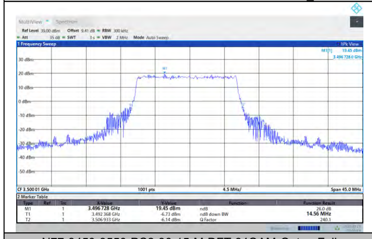
N77-3450-3550-PC2-30-15-M-DFT-64QAM-Outer_Full
