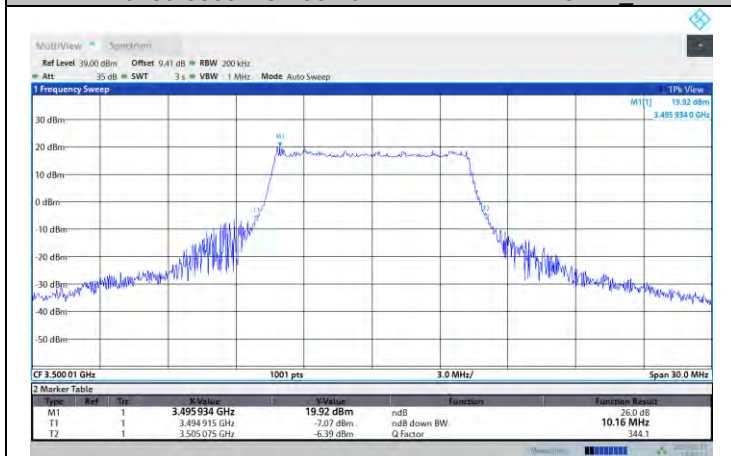
N77-3450-3550-PC2-30-10-M-DFT-16QAM-Outer_Full
