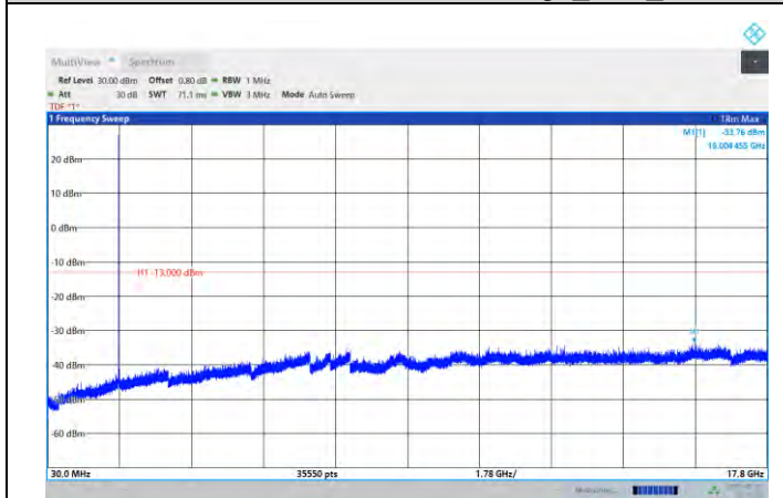
N66-PC3-5MHz-H-DFT-QPSK-Edge_1RB_Left
