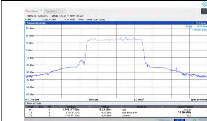
N66-PC3-20MHz-M-DFT-64QAM-Outter_Full
