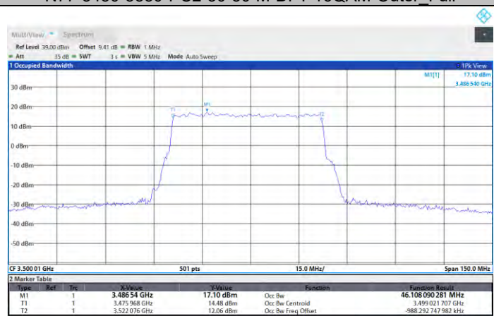
N77-3450-3550-PC2-30-50-M-DFT-256QAM-Outer_Full
