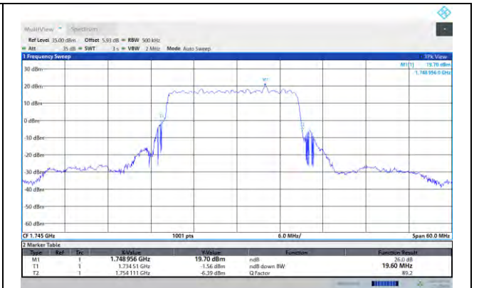
N66-PC3-20MHz-M-DFT-PI2BPSK-Outter_Full
