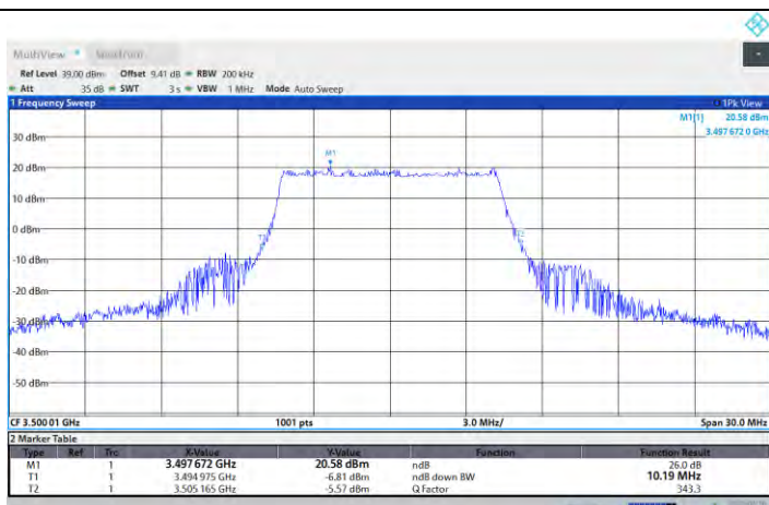
N77-3450-3550-PC2-30-10-M-DFT-QPSK-Outer_Full
