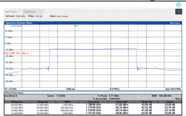
N66-PC3-40MHz-L-DFT-QPSK-Outer Full
