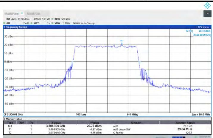
N77-3450-3550-PC2-30-30-M-DFT-PI2BPSK-Outer_Full
