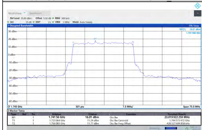
N66-PC3-25MHz-M-DFT-16QAM-Outer_Full
