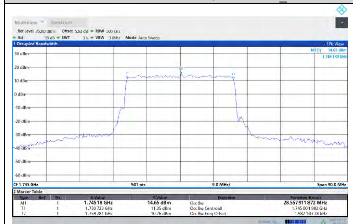
N66-PC3-30MHz-M-DFT-64QAM-Outer_Full
