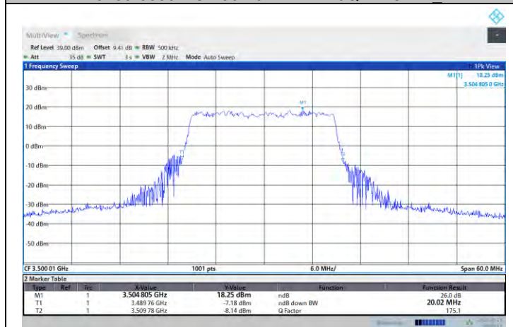
N77-3450-3550-PC2-30-20-M-DFT-256QAM-Outer_Full
