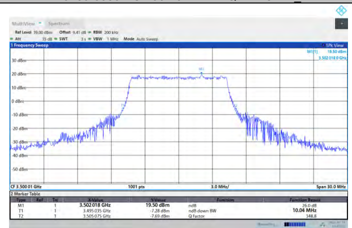
N77-3450-3550-PC2-30-10-M-DFT-64QAM-Outer_Full
