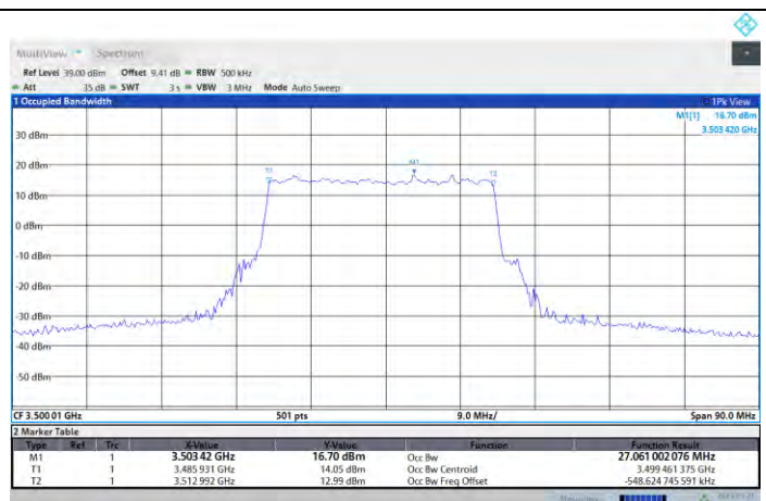
N77-3450-3550-PC2-30-30-M-DFT-256QAM-Outer_Full
