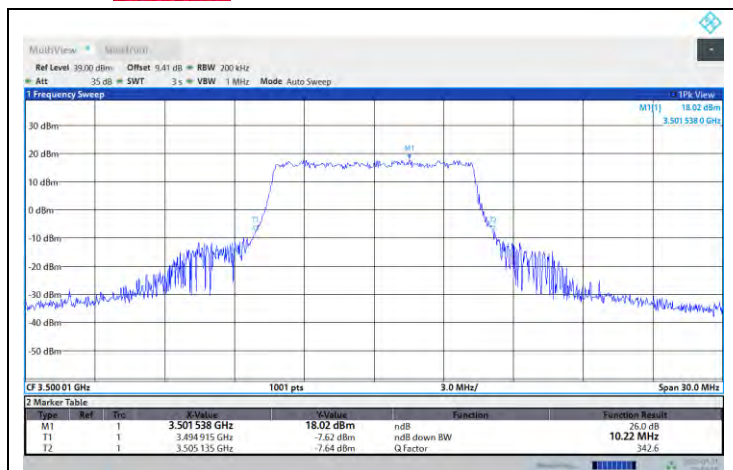
N77-3450-3550-PC2-30-10-M-DFT-256QAM-Outer_Full
