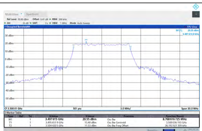
N77-3450-3550-PC2-30-10-M-DFT-QPSK-Outer_Full
