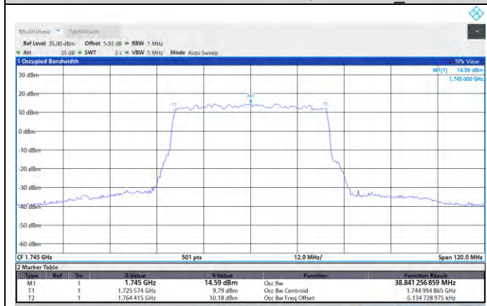
N66-PC3-40MHz-M-DFT-256QAM-Outer_Full
