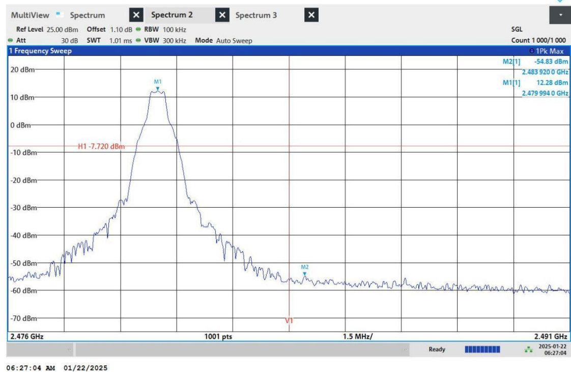
DH5_ANT7_High_2480
