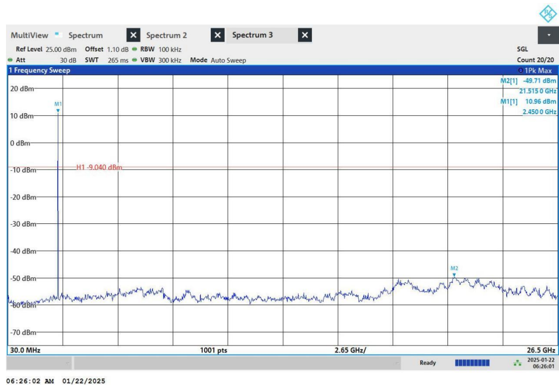
DH5_ANT7_2441_30~26500
