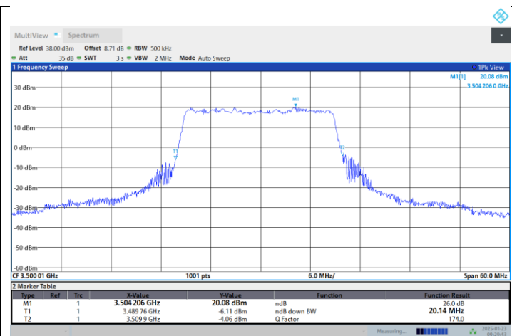
N77-3450-3550-PC2-30-20-M-DFT-QPSK-Outer Full
