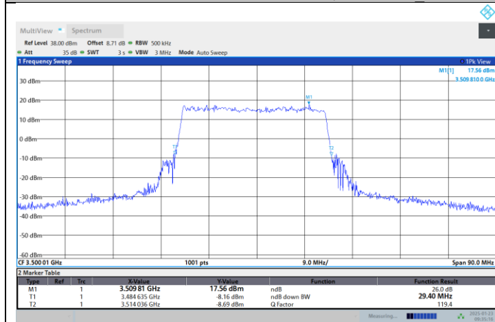
N77-3450-3550-PC2-30-30-M-DFT-64QAM-Outer_Full
