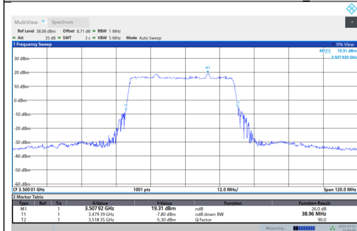
N77-3450-3550-PC2-30-40-M-DFT-PI2BPSK-Outer_Full
