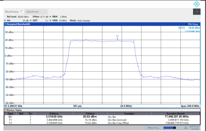
N77-3450-3550-PC2-30-80-M-DFT-PI2BPSK-Outer Full
