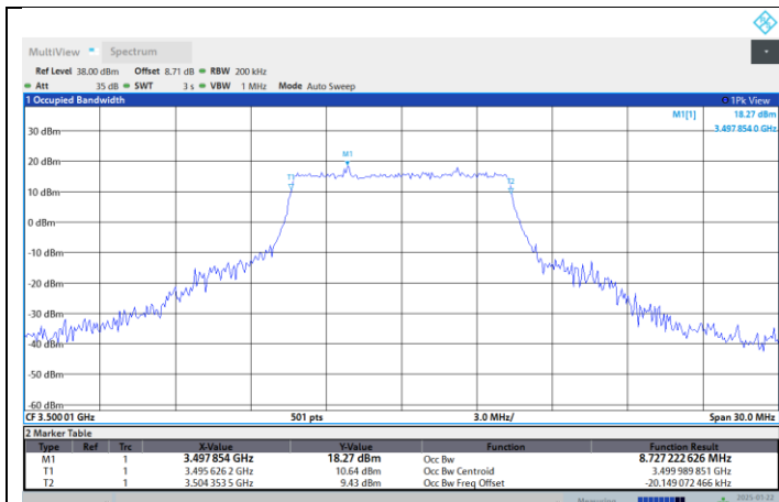
N77-3450-3550-PC2-30-10-M-DFT-PI2BPSK-Outer_Full
