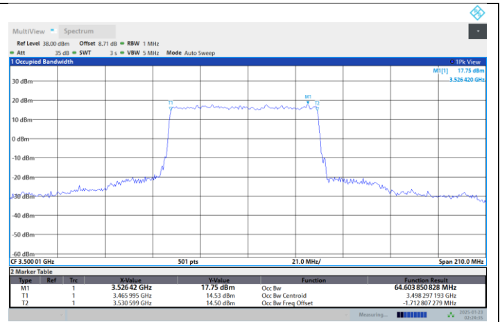
N77-3450-3550-PC2-30-70-M-DFT-QPSK-Outer Full
