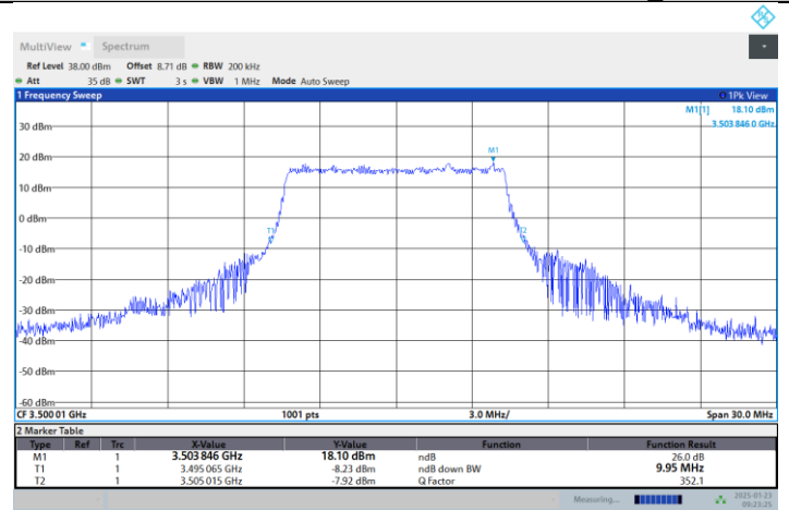
N77-3450-3550-PC2-30-10-M-DFT-64QAM-Outer_Full
