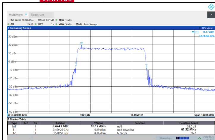
N77-3450-3550-PC2-30-60-M-DFT-64QAM-Outer_Full
