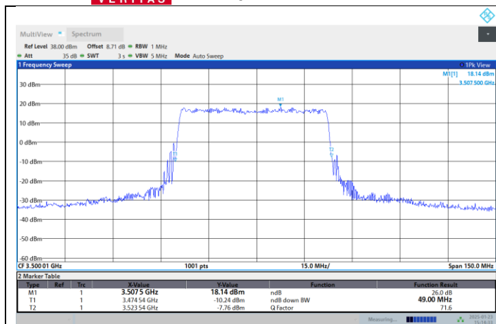
N77-3450-3550-PC2-30-50-M-DFT-64QAM-Outer_Full
