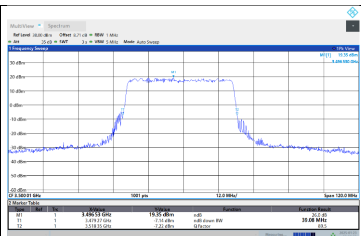
N77-3450-3550-PC2-30-40-M-DFT-64QAM-Outer_Full
