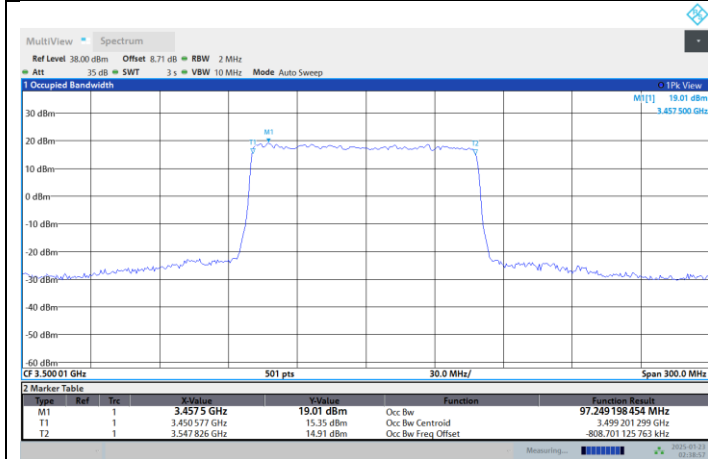
N77-3450-3550-PC2-30-100-M-DFT-QPSK-Outer Full
