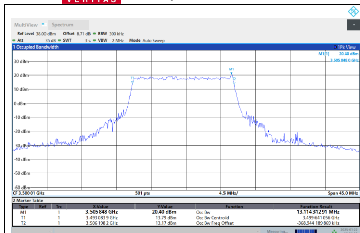
N77-3450-3550-PC2-30-15-M-DFT-QPSK-Outer_Full
