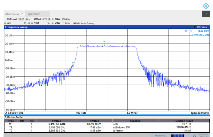
N77-3450-3550-PC2-30-10-M-DFT-QPSK-Outer_Full
