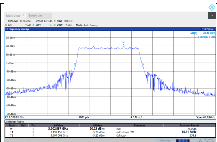
N77-3450-3550-PC2-30-15-M-DFT-PI2BPSK-Outer_Full
