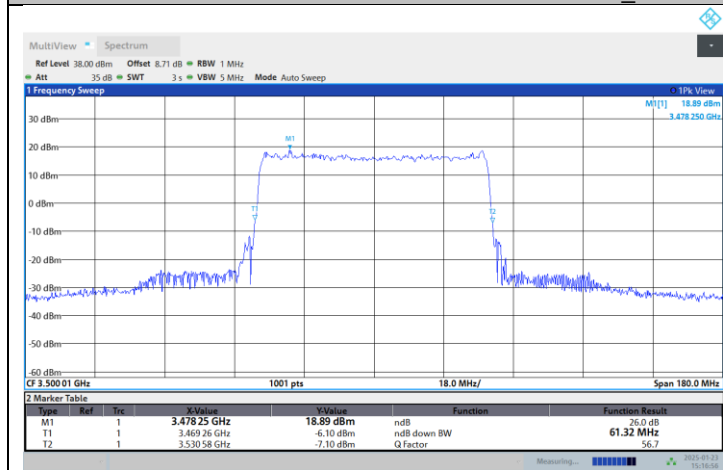
N77-3450-3550-PC2-30-60-M-DFT-QPSK-Outer_Full
