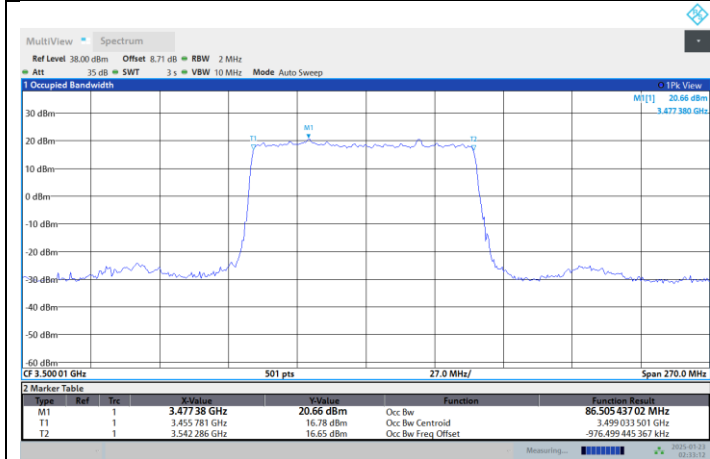
N77-3450-3550-PC2-30-90-M-DFT-PI2BPSK-Outer_Full
