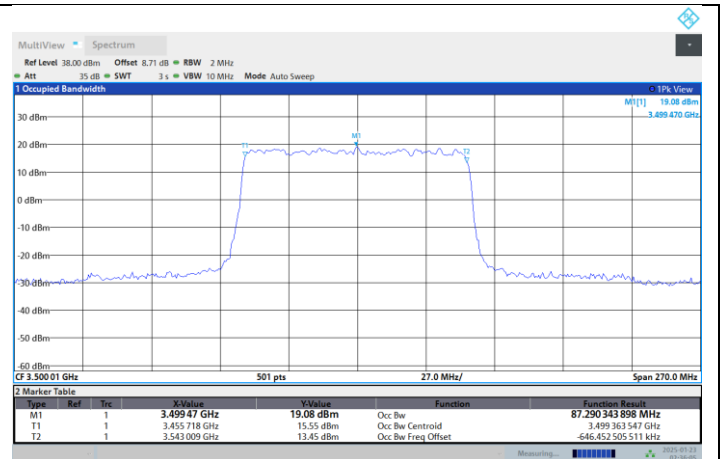
N77-3450-3550-PC2-30-90-M-DFT-64QAM-Outer Full
