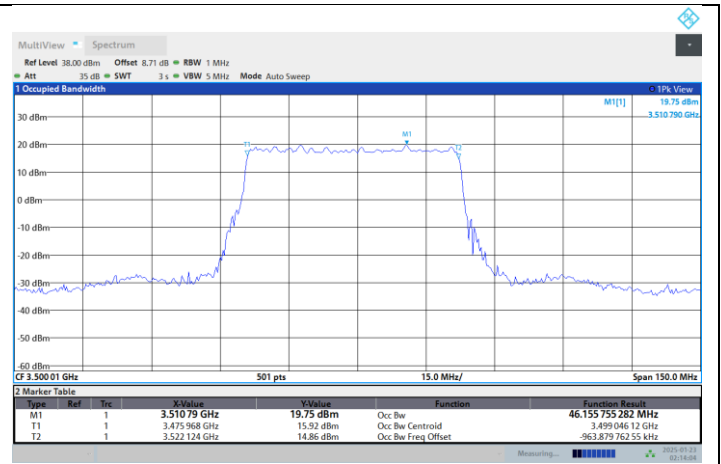
N77-3450-3550-PC2-30-50-M-DFT-PI2BPSK-Outer_Full
