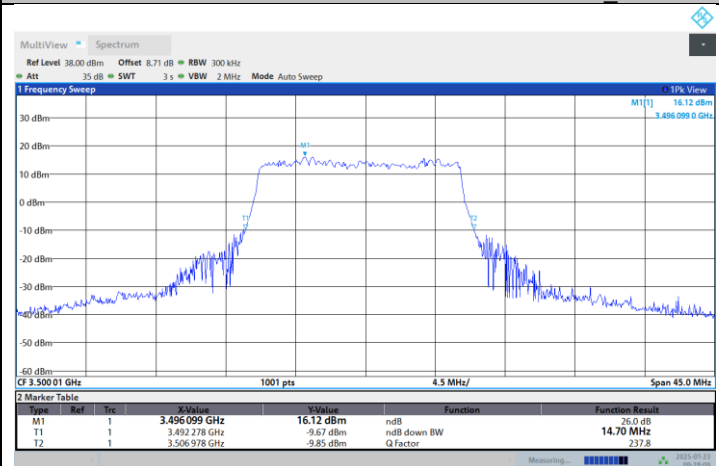
N77-3450-3550-PC2-30-15-M-DFT-256QAM-Outer_Full
