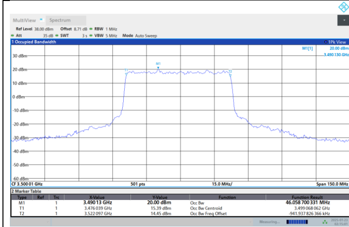
N77-3450-3550-PC2-30-50-M-DFT-QPSK-Outer_Full
