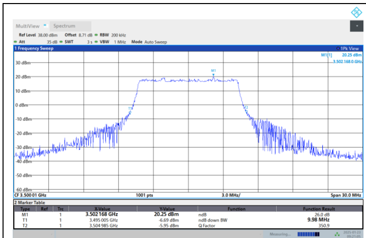
N77-3450-3550-PC2-30-10-M-DFT-PI2BPSK-Outer_Full
