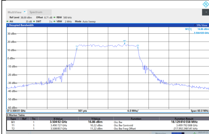
N77-3450-3550-PC2-30-20-M-DFT-256QAM-Outer_Full
