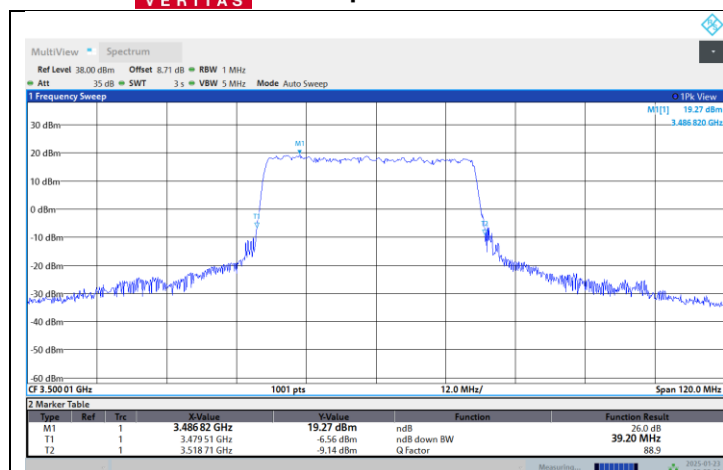
N77-3450-3550-PC2-30-40-M-DFT-16QAM-Outer_Full
