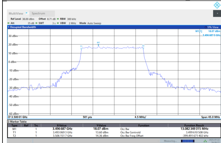
N77-3450-3550-PC2-30-15-M-DFT-64QAM-Outer_Full
