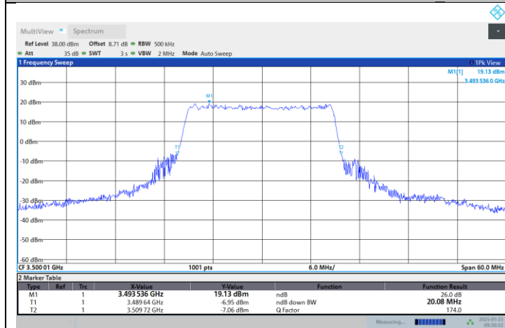
N77-3450-3550-PC2-30-20-M-DFT-16QAM-Outer Full
