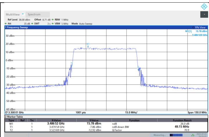
N77-3450-3550-PC2-30-50-M-DFT-256QAM-Outer_Full
