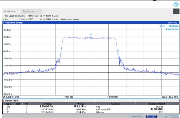
N77-3450-3550-PC2-30-40-M-DFT-QPSK-Outer_Full
