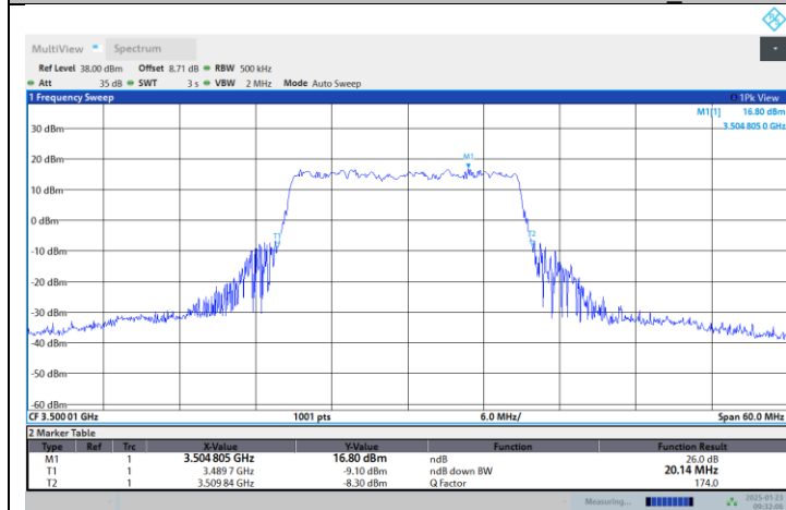
N77-3450-3550-PC2-30-20-M-DFT-256QAM-Outer Full
