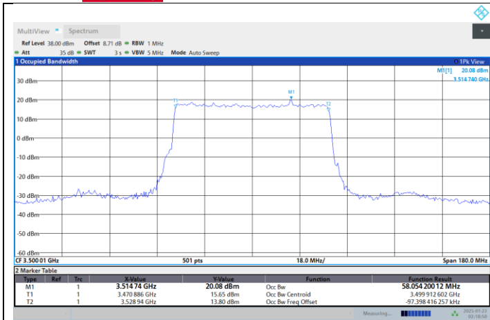
N77-3450-3550-PC2-30-60-M-DFT-PI2BPSK-Outer_Full
