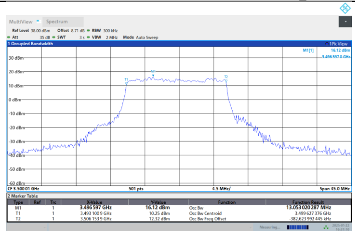
N77-3450-3550-PC2-30-15-M-DFT-256QAM-Outer_Full
