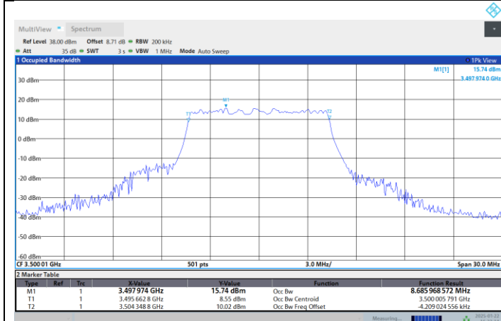
N77-3450-3550-PC2-30-10-M-DFT-256QAM-Outer_Full
