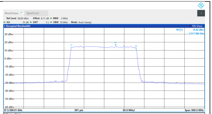
N77-3450-3550-PC2-30-100-M-DFT-256QAM-Outer_Full
