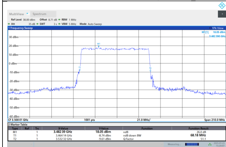
N77-3450-3550-PC2-30-70-M-DFT-PI2BPSK-Outer_Full
