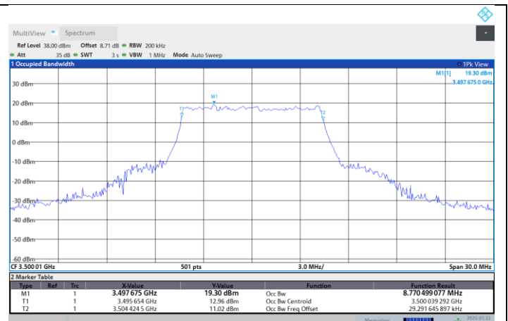
N77-3450-3550-PC2-30-10-M-DFT-QPSK-Outer_Full
