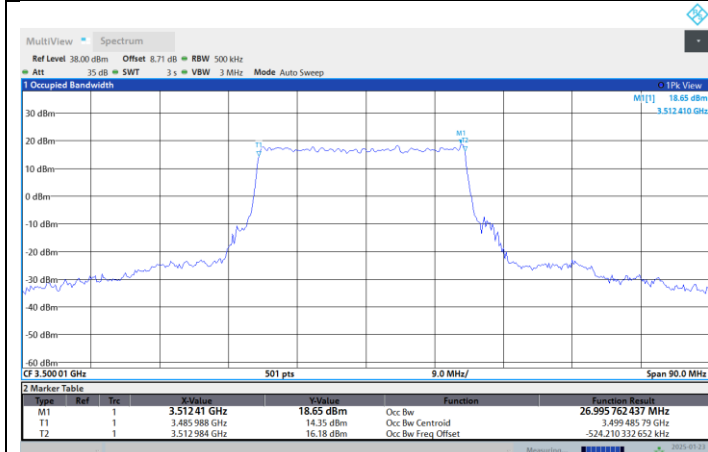
N77-3450-3550-PC2-30-30-M-DFT-QPSK-Outer_Full
