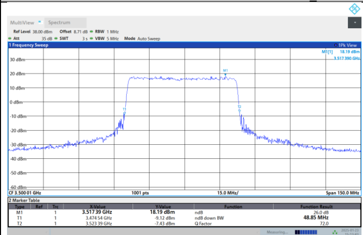
N77-3450-3550-PC2-30-50-M-DFT-16QAM-Outer_Full
