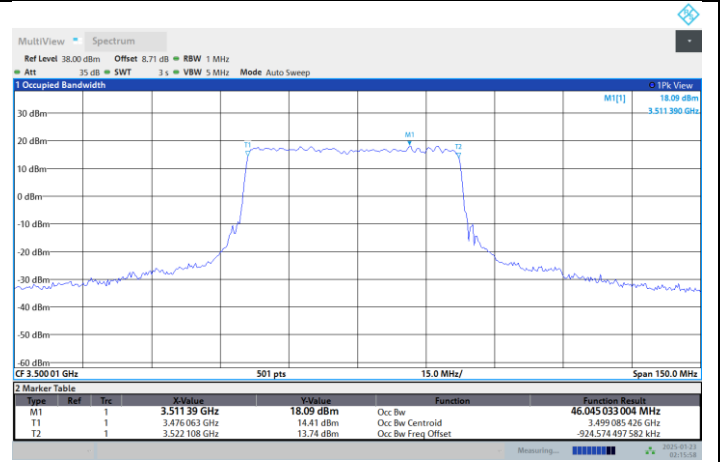
N77-3450-3550-PC2-30-50-M-DFT-16QAM-Outer_Full
