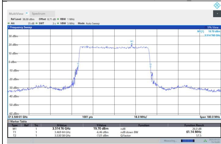
N77-3450-3550-PC2-30-60-M-DFT-PI2BPSK-Outer_Full
