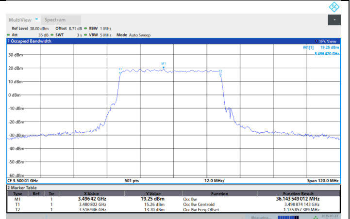
N77-3450-3550-PC2-30-40-M-DFT-64QAM-Outer Full
