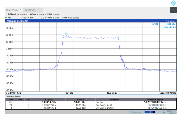
N77-3450-3550-PC2-30-60-M-DFT-64QAM-Outer_Full
