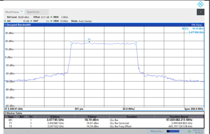
N77-3450-3550-PC2-30-100-M-DFT-16QAM-Outer Full
