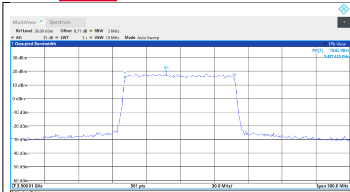
N77-3450-3550-PC2-30-100-M-DFT-64QAM-Outer_Full
