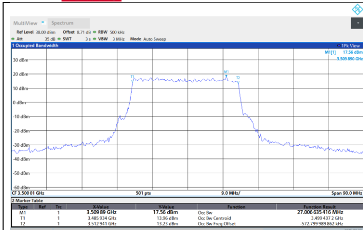
N77-3450-3550-PC2-30-30-M-DFT-64QAM-Outer Full
