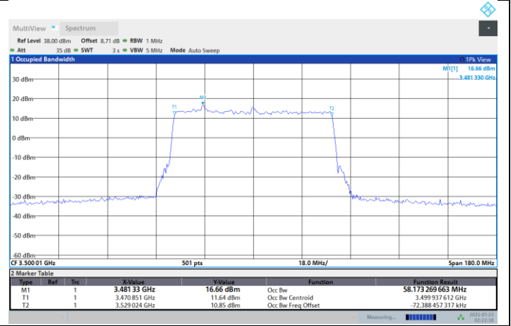
N77-3450-3550-PC2-30-60-M-DFT-256QAM-Outer_Full
