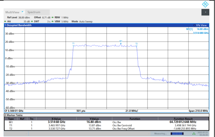
N77-3450-3550-PC2-30-70-M-DFT-64QAM-Outer Full
