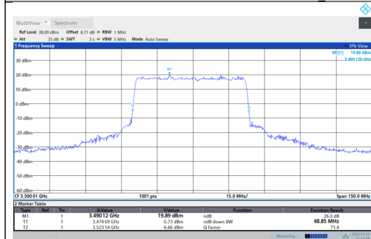
N77-3450-3550-PC2-30-50-M-DFT-QPSK-Outer_Full
