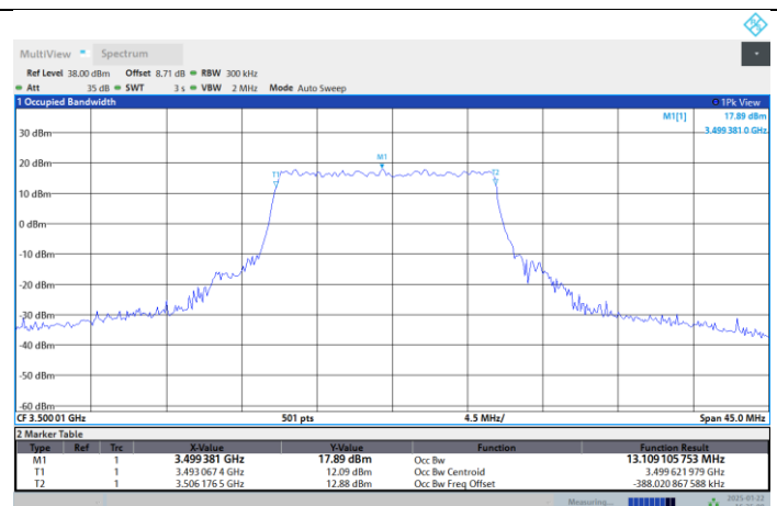
N77-3450-3550-PC2-30-15-M-DFT-16QAM-Outer_Full
