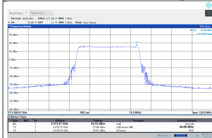
N77-3450-3550-PC2-30-40-M-DFT-256QAM-Outer_Full
