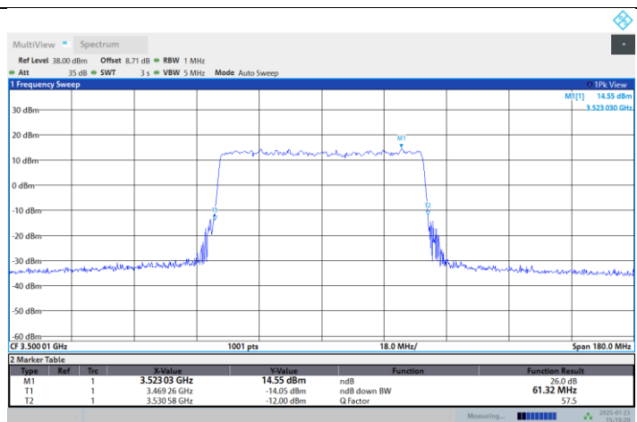
N77-3450-3550-PC2-30-60-M-DFT-256QAM-Outer_Full
