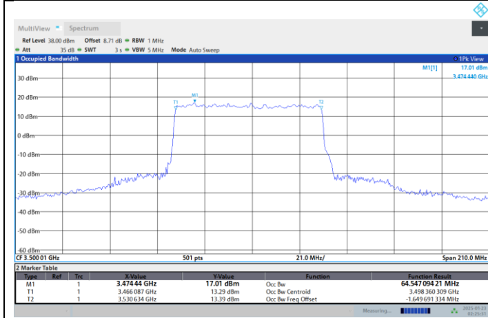
N77-3450-3550-PC2-30-70-M-DFT-16QAM-Outer Full
