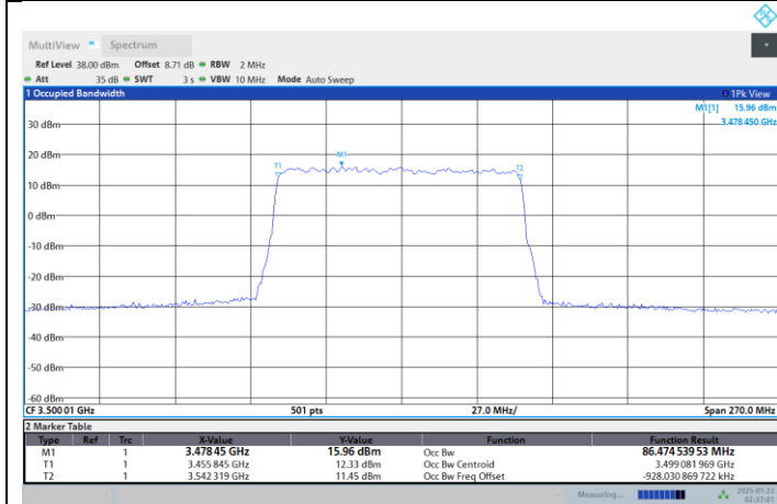
N77-3450-3550-PC2-30-90-M-DFT-256QAM-Outer Full
