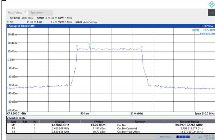
N77-3450-3550-PC2-30-70-M-DFT-256QAM-Outer Full
