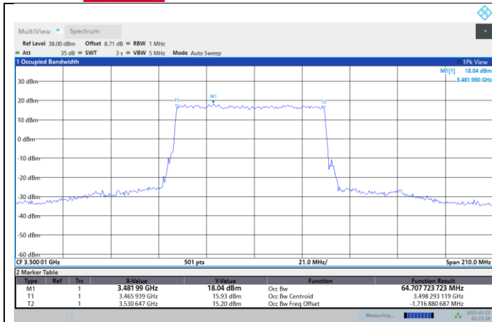
N77-3450-3550-PC2-30-70-M-DFT-PI2BPSK-Outer Full
