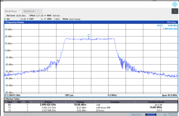
N77-3450-3550-PC2-30-15-M-DFT-16QAM-Outer_Full
