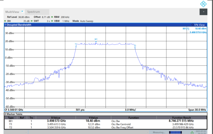
N77-3450-3550-PC2-30-10-M-DFT-64QAM-Outer_Full
