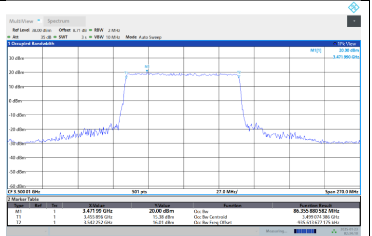
N77-3450-3550-PC2-30-90-M-DFT-QPSK-Outer_Full
