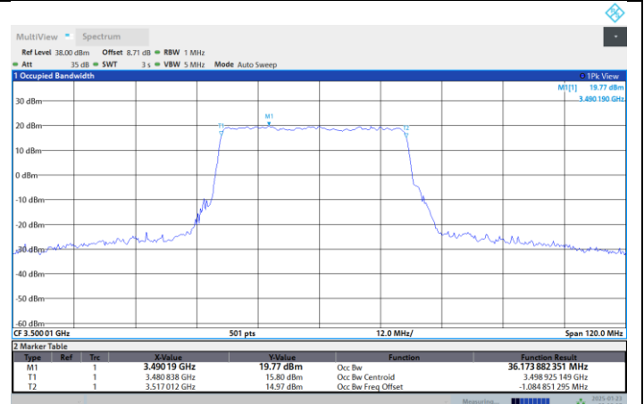
N77-3450-3550-PC2-30-40-M-DFT-QPSK-Outer Full
