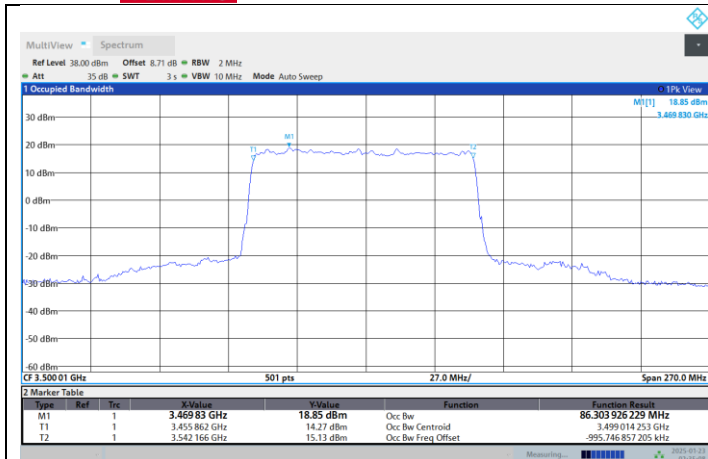
N77-3450-3550-PC2-30-90-M-DFT-16QAM-Outer Full
