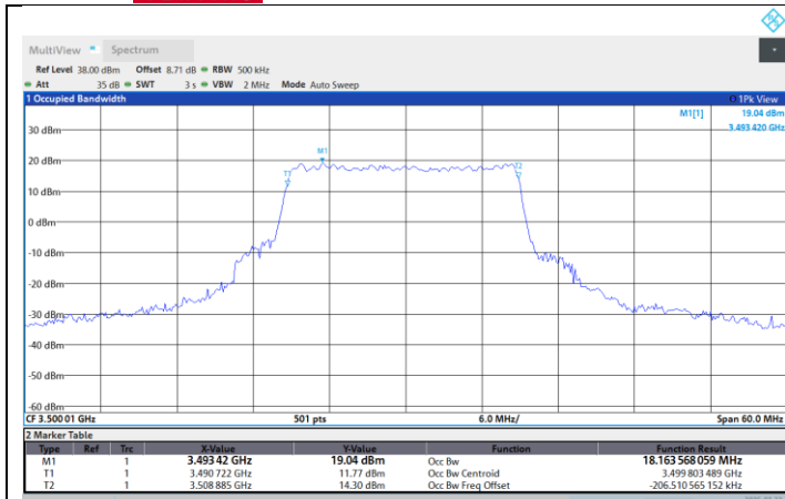
N77-3450-3550-PC2-30-20-M-DFT-16QAM-Outer_Full
