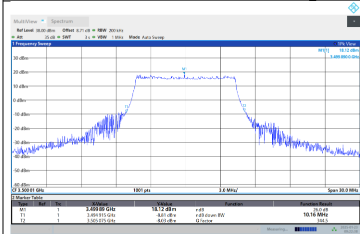
N77-3450-3550-PC2-30-10-M-DFT-16QAM-Outer_Full
