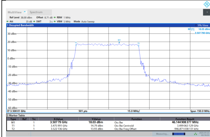
N77-3450-3550-PC2-30-50-M-DFT-64QAM-Outer_Full
