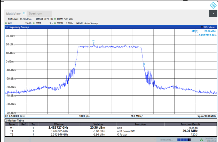
N77-3450-3550-PC2-30-30-M-DFT-PI2BPSK-Outer Full
