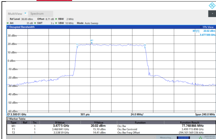
N77-3450-3550-PC2-30-80-M-DFT-QPSK-Outer_Full
