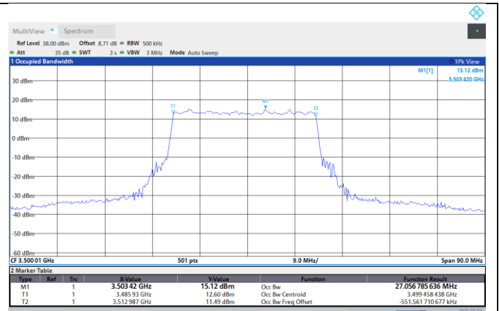
N77-3450-3550-PC2-30-30-M-DFT-256QAM-Outer Full
