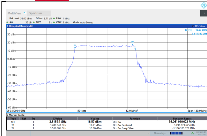
N77-3450-3550-PC2-30-40-M-DFT-256QAM-Outer_Full
