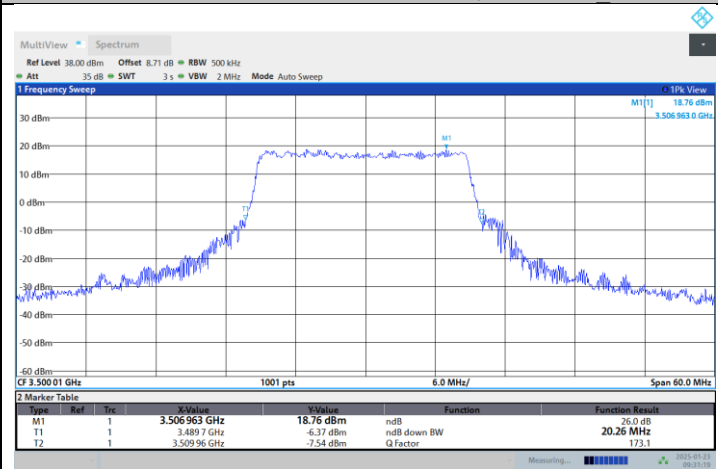
N77-3450-3550-PC2-30-20-M-DFT-64QAM-Outer Full
