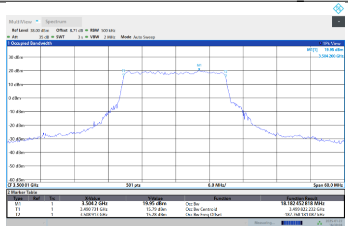
N77-3450-3550-PC2-30-20-M-DFT-QPSK-Outer_Full
