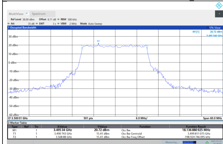
N77-3450-3550-PC2-30-20-M-DFT-PI2BPSK-Outer_Full
