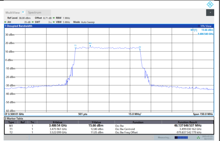
N77-3450-3550-PC2-30-50-M-DFT-256QAM-Outer_Full
