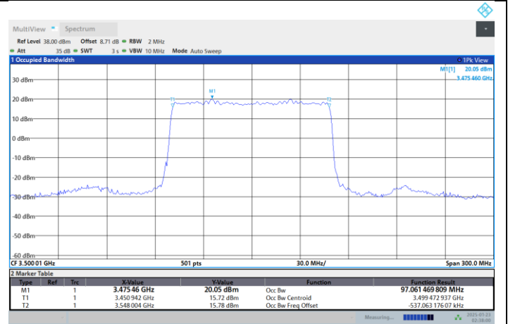
N77-3450-3550-PC2-30-100-M-DFT-PI2BPSK-Outer Full
