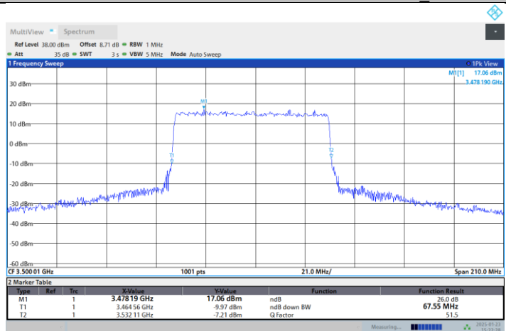
N77-3450-3550-PC2-30-70-M-DFT-64QAM-Outer_Full
