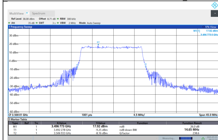
N77-3450-3550-PC2-30-15-M-DFT-64QAM-Outer_Full
