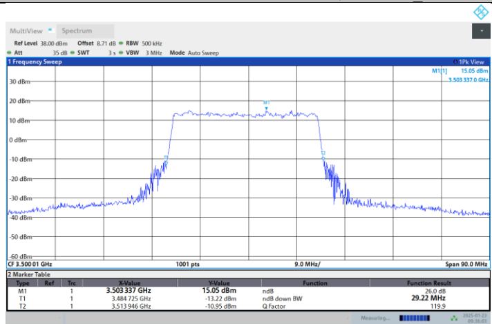
N77-3450-3550-PC2-30-30-M-DFT-256QAM-Outer_Full
