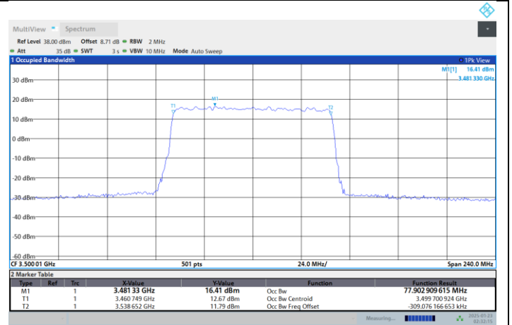
N77-3450-3550-PC2-30-80-M-DFT-256QAM-Outer_Full
