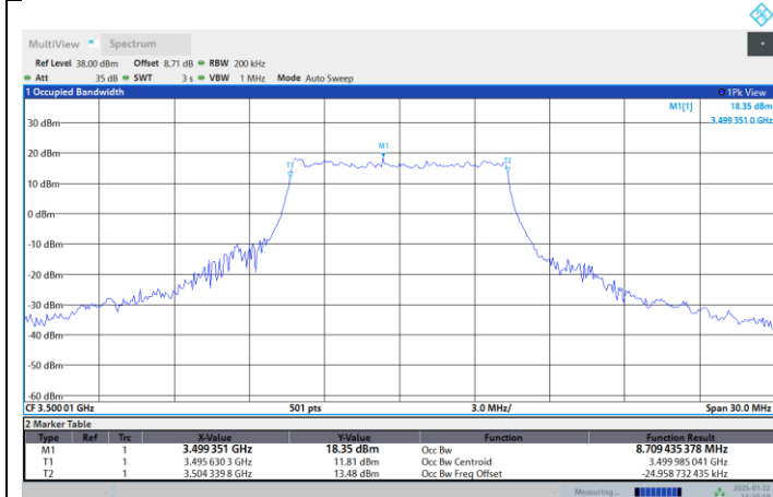
N77-3450-3550-PC2-30-10-M-DFT-16QAM-Outer_Full
