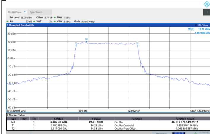
N77-3450-3550-PC2-30-40-M-DFT-16QAM-Outer Full
