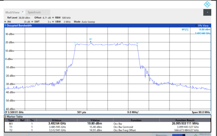
N77-3450-3550-PC2-30-30-M-DFT-P12BPSK-Outer_Full
