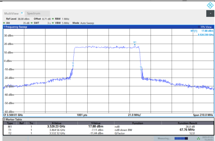
N77-3450-3550-PC2-30-70-M-DFT-QPSK-Outer_Full
