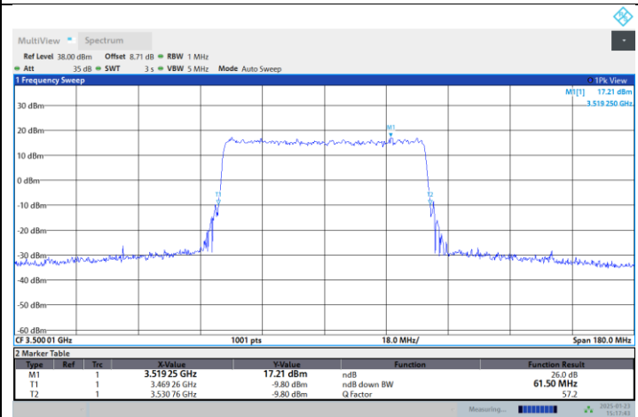
N77-3450-3550-PC2-30-60-M-DFT-16QAM-Outer_Full
