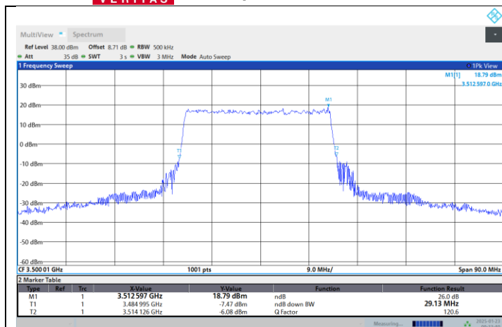
N77-3450-3550-PC2-30-30-M-DFT-QPSK-Outer_Full
