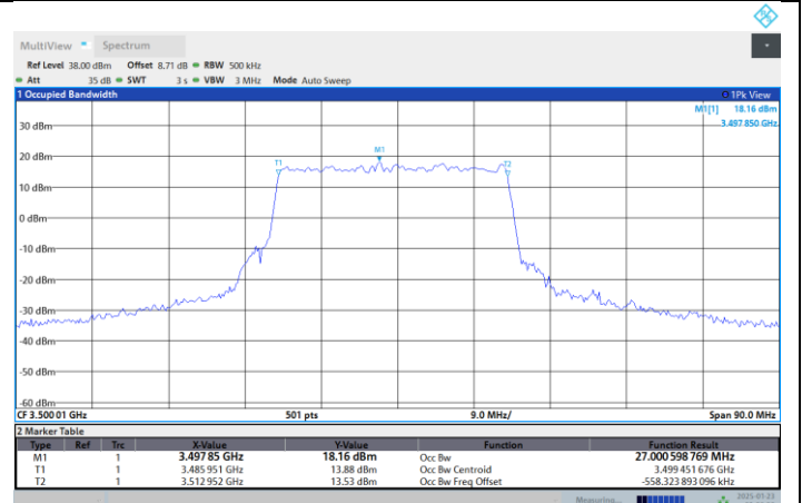
N77-3450-3550-PC2-30-30-M-DFT-16QAM-Outer_Full
