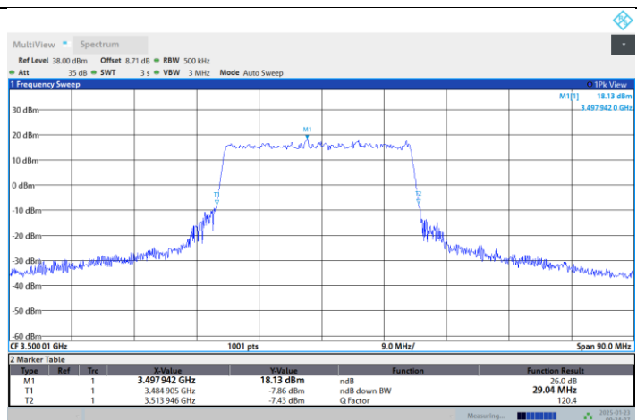
N77-3450-3550-PC2-30-30-M-DFT-16QAM-Outer_Full
