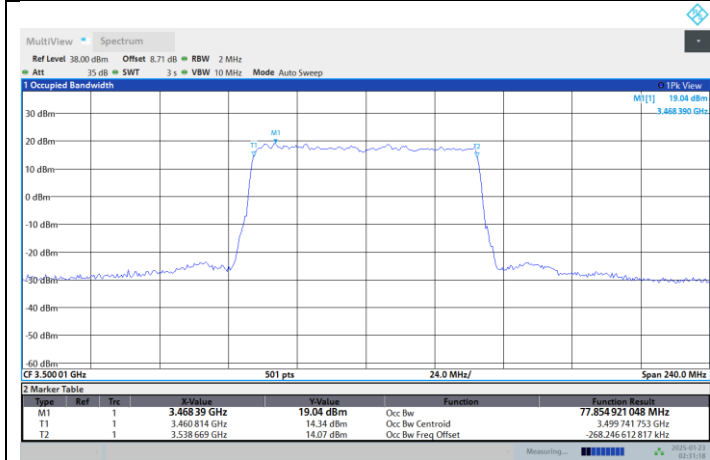
N77-3450-3550-PC2-30-80-M-DFT-64QAM-Outer_Full
