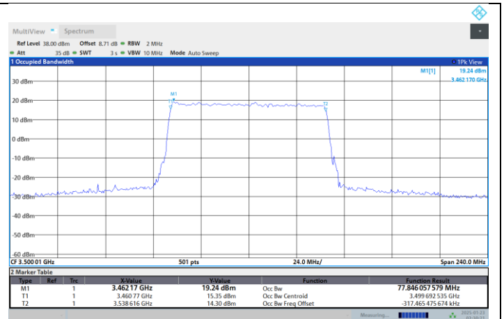
N77-3450-3550-PC2-30-80-M-DFT-16QAM-Outer_Full
