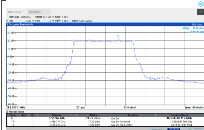
N77-3450-3550-PC2-30-40-M-DFT-PI2BPSK-Outer Full
