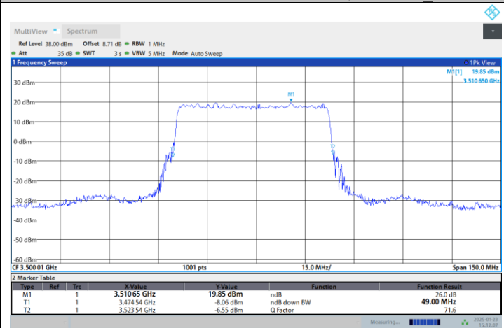
N77-3450-3550-PC2-30-50-M-DFT-PI2BPSK-Outer_Full
