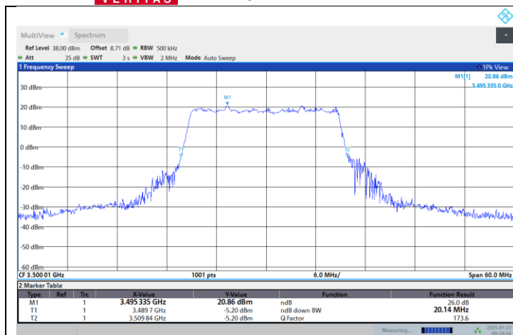
N77-3450-3550-PC2-30-20-M-DFT-PI2BPSK-Outer Full
