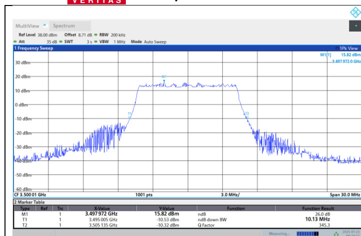
N77-3450-3550-PC2-30-10-M-DFT-256QAM-Outer_Full
