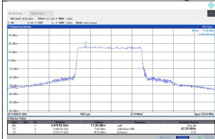
N77-3450-3550-PC2-30-70-M-DFT-16QAM-Outer_Full
