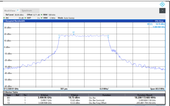
N77-3450-3550-PC2-30-20-M-DFT-64QAM-Outer_Full
