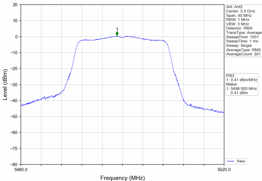
802.11ac(VHT20)_LCH_5500MHz_Ant2_NTNV
