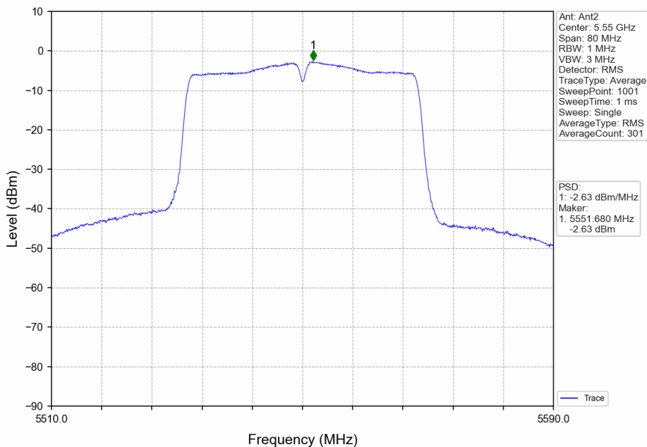
802.11ac(VHT40)_MCH_5550MHz_Ant2_NTNV
