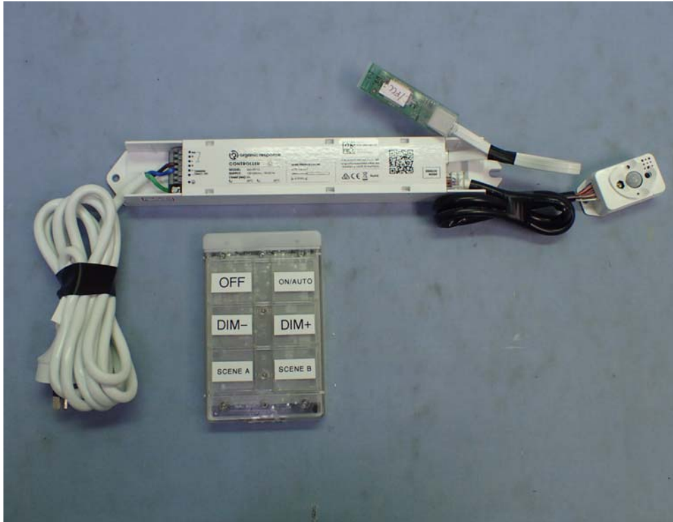
Figure 2 Controller P2UL, General Appearance
