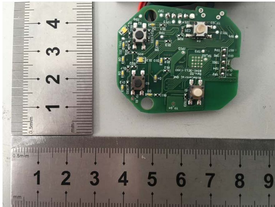
EUT – IC Chips View
