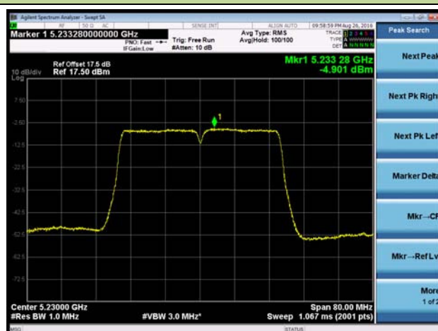
Channel 46 (5230MHz)
