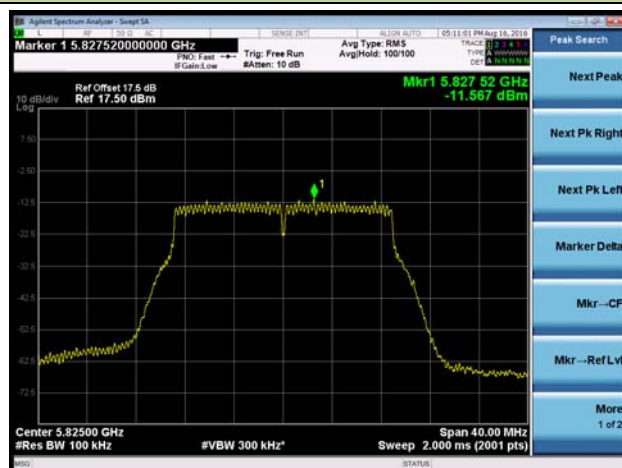
Channel 165 (5825MHz)
