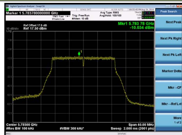
802.11n-HT40 Power Spectral Density - Ant 1
