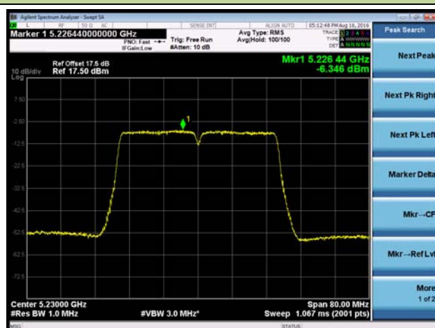
Channel 46 (5230MHz)
