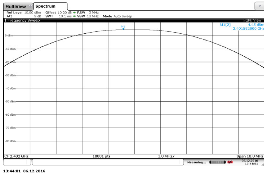
Figure 7.4.2-1: Power Output - LCH
