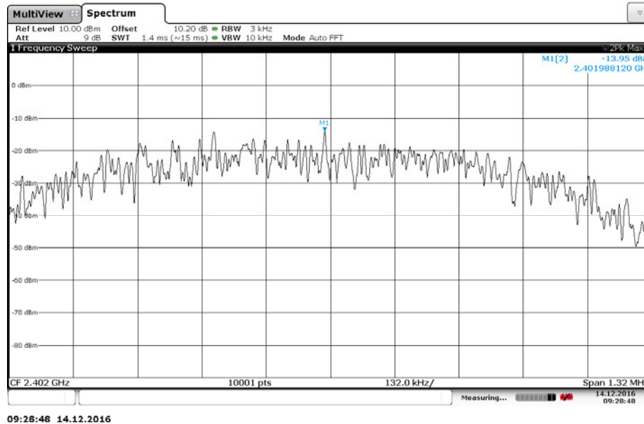
Figure 7.6.2-1: PSD Plot –LCH
