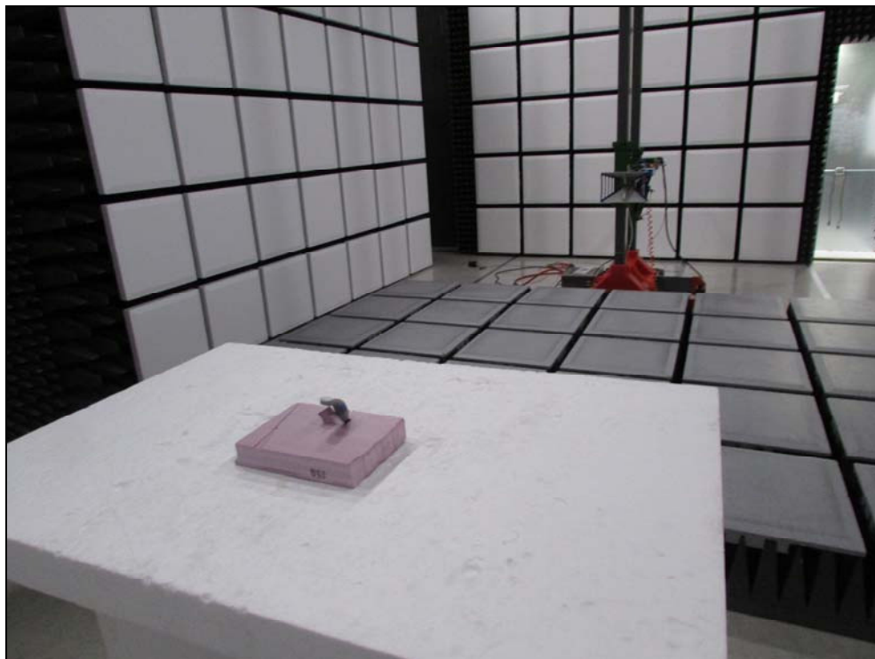
Figure 2: Above 1GHz – Rear View
