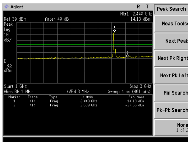
1GHz ~3GHz
