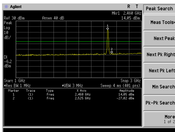
1GHz~3GHz
