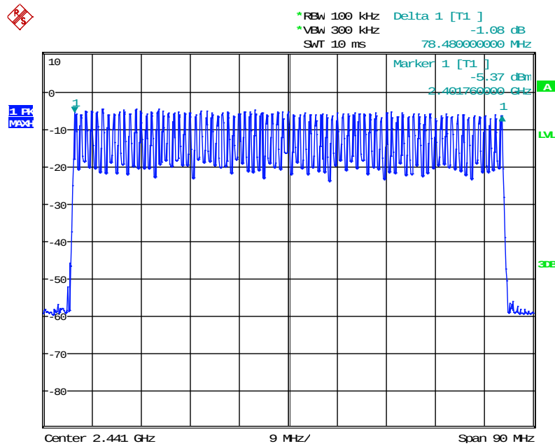
Number of hopping channels (GFSK Mode)
