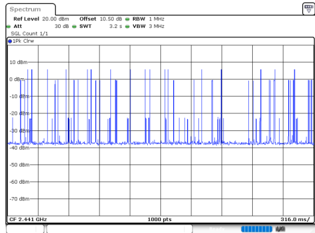
2DH3_Hopping
