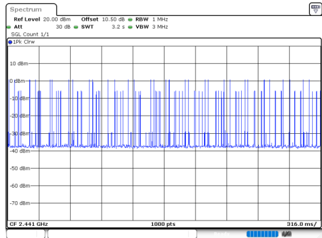
2DH1_Hopping
