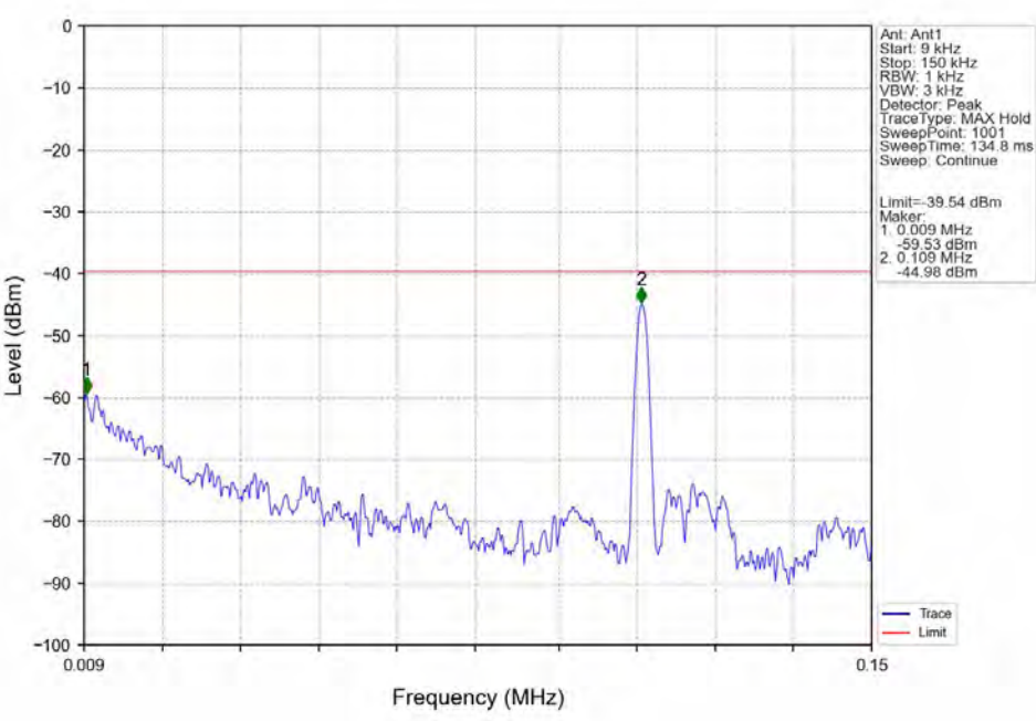
\pi/4 DQPSK_2DH5_LCH_2402MHz_Ant1_NTNV
