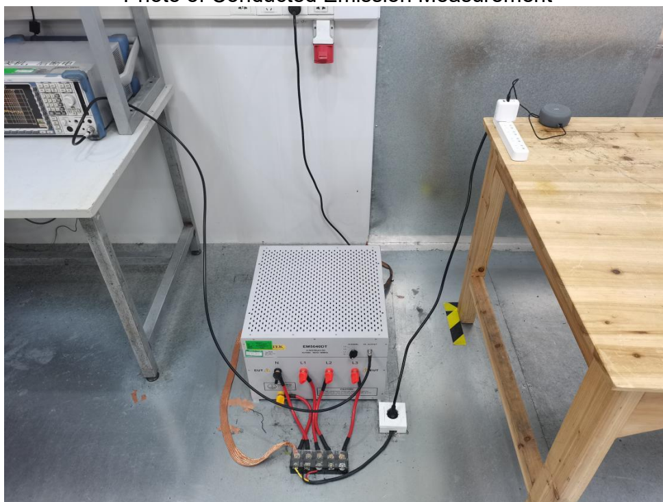
FCC ID: 2AJQ7MIST Photo of Conducted Emission Measurement
