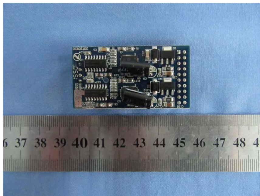
EUT – SUB Board Bottom View
