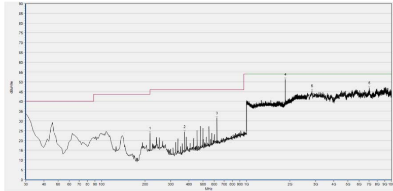
(Plot C.1: 30MHz to 10GHz, Antenna Horizontal @ Profile 0, channel 50)
