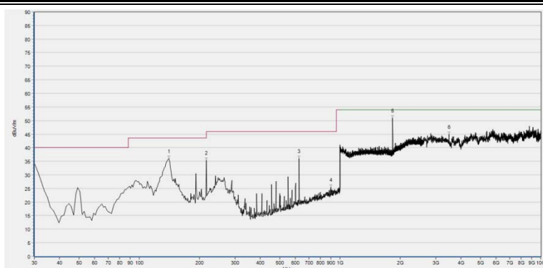
(Plot B.1: 30MHz to 10GHz, Antenna Horizontal, channel 26)
